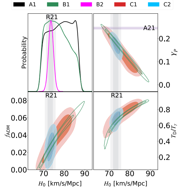
FIG. 2. Constraints on parameters from datasets 1 and 2 given models A , B , and C (see Tables I and II). Top left panel: the (unnormalized) posterior probability density of H_0 . Other panels: the 68% and 95% contours of equal probability density in the H_0 - Y_p , H_0 - f_{\text{ADM}} , and H_0 - T_D/T_\gamma planes. The gray band “R21” shows the 1\sigma and 2\sigma constraint on H_0 from R21. The purple band “A21” shows the same for Y_p from ([157] hereafter A21).
