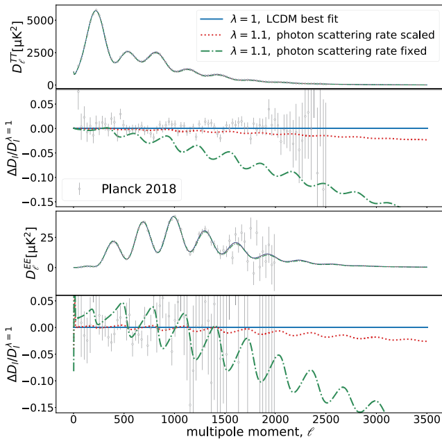
FIG. 1. CMB temperature (TT) and polarization (EE) power spectra with (red and green) and without (blue) scaling by \lambda = 1.1 from the best-fit \Lambda CDM model for dataset 1. Both \lambda = 1.1 cases are scaled by use of the mirror world dark sector, with (red) and without (green) scaling of the photon scattering rate. Data points are from Planck 2018 [147]. Fractional differences with the best-fit \Lambda CDM model are shown in the second and bottom panels.
