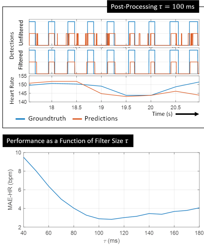
Fig. 2: Illustration of heartbeat filtering and heart rate computation. [Top] Filtering results by applying a median filter with a filter size \tau = 100 ms including estimated heart rate. [Bottom] The MAE for heart rate from the training data as a function of the filter size \tau . A value around \tau = 100 ms seems to be optimal in this case yielding a training error under 3 beats per minute.
