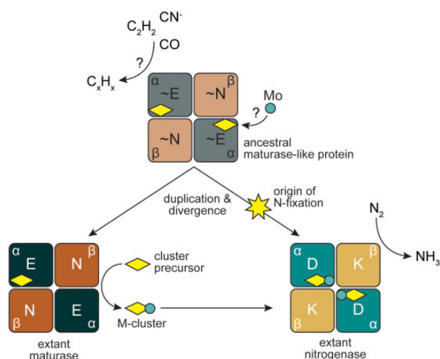
Fig. 4. —Proposed model for the origins and functional divergence of maturated and nitrogenase proteins. An ancestral maturase-like protein (~NifEN, gray and light brown), incapable of reducing N_2 , may have otherwise reduced various carbon-containing substrates and/or played a role in cluster (yellow diamond) biosynthesis. The ancestor may have been capable of incorporating molybdenum (teal circle) into the cluster. Duplication of the encoding ancestral genes and functional divergence would then have yielded canonical maturated (NifEN, dark green and brown) and nitrogenase (NifDK, teal and yellow) proteins. Maturated proteins would have specialized to provide a scaffold for the maturation of the nitrogenase cluster precursor (yellow diamond) to the nitrogenase active-site M-cluster (yellow diamond with teal circle). In parallel, tuning of the ancestral peptide environment along a divergent lineage would have spurred the origin of N_2 reduction and specialization of nitrogenases for a solely catalytic role in nitrogen fixation. Protein components of the \alpha_2\beta_2 heterotetrameric nitrogenase and maturated structures are labeled.
