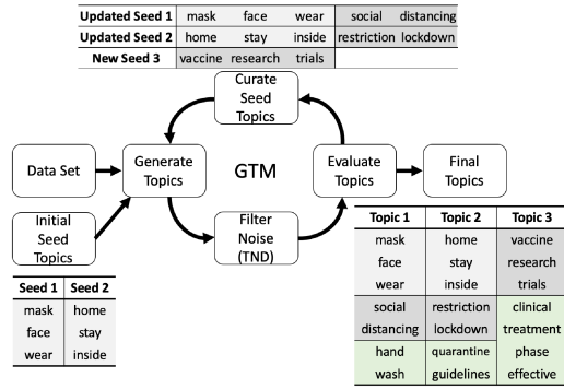
Figure 1: GTM Flow Chart. Words are shaded differently by each round they are added to the topic.
