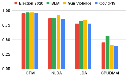
Figure 5: Topic diversity comparison.
