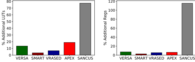
(a) Additional HW overhead (%) in Number of Look-Up Tables (b) Additional HW overhead (%) in Number of Registers Fig. 9. Hardware overhead comparisons with other low-end security architectures.
