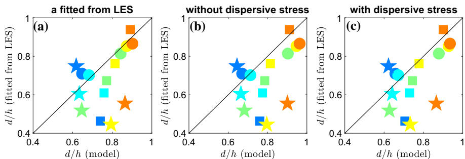
Fig. 14 Comparisons between the reference d/h obtained from fitting the log-law to U in the ISL (see Table 1) and models for d/h . a d/h is modelled based on Eq. 19 using attenuation coefficients a fitted from LES; b d/h based on Eq. 19 using a modelled by the first equality of Eq. 14 without correcting for the effect of dispersive stress on a ; c the same as (b), except correcting for the effect of dispersive stress on a
