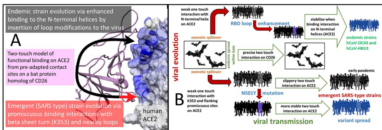
Figure 11. A functional evolutionary model of SARS-type and endemic viral protein binding interactions during zoonotic spillover. (A) The two-touch interaction model consists of a combination of evolutionary conserved ACE2 interactions at the N-terminal helices likely preadapted from its interaction with the SAMLI 291-5 motif on CD26 (shown with black arrow) and a promiscuous, dynamically complex interaction with K353 and nearby sites at Q325 and AAQPFL 386-392 (shown with red arrow), likely preadapted from its interaction with SS 333-334 on CD26. (B) Given the conserved nature of viral receptor binding across the diversity of strains we surveyed, we hypothesize these regions of the virus are most likely responsible for past and present instances of zoonotic spillover to humans. The more pathogenic SARS-like outbreaks associated with ACE2 seem to develop transient dynamics of N501 that involve promiscuous interactions at three co-located sites mentioned above. This may create a temporary 'slippery' two touch interaction with the ACE2 target that stabilizes over evolutionary time. In the much more transmissible new variant strains (B.1.1.7, B.1.351, and P.1), the promiscuous interactions are mostly lost, favoring a much more stable binding interaction with K353 alone. In both endemic strains, we observe the evolution of enhanced binding to the N-terminal helices of ACE2 through the evolution of enhanced loop structure on the corresponding interface of the viral receptor binding domain.
