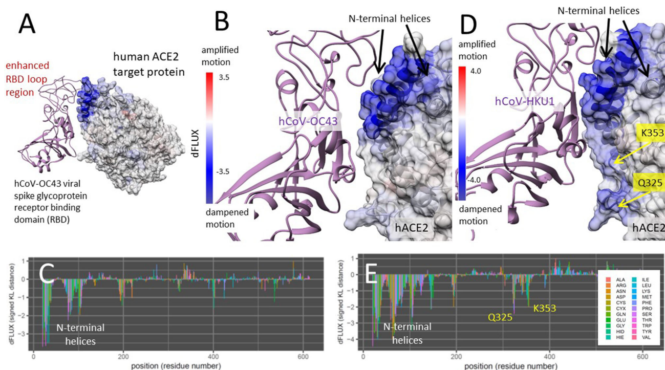
Figure 7. DROIDS binding signature of dampened atom fluctuations in human ACE2 receptor proteins upon interaction with two human endemic strains hCoV-OC43 and hCoV-HKU1 glycoprotein (modeled from PDB: 6ohw, 5gnb and 6m17). Here we show color mapping (A, B, D) and sequence positional plotting (C, E) of dampening of atom motion on the viral RBD-protein target interface in blue for (A–C) the targeting of ACE2 by the most benign strain hCoV-OC43 and (D, E) its less benign counterpart hCoV-HKU1. The sequence profile of the KL divergence between viral bound and unbound target proteins produces strong negative peak indicating key residue binding interactions (C, E) with the N-terminal helices on ACE2 and (E) moderate interactions with K353 and Q325 observed only in hCoV-HKU1.
