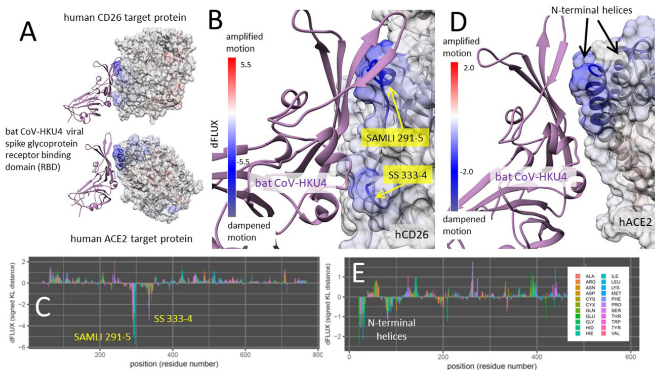
Figure 8. DROIDS binding signature of dampened atom fluctuations in human CD26 and ACE2 receptor proteins upon interaction with the bat progenitor strain batCoV-HKU4 glycoprotein (modeled from PDB: 4qzv and 6m17). Here we show color mapping (A, B, D) and sequence positional plotting (C, E) of dampening of atom motion on the viral RBD-protein target interface in blue for (A–C) its known targeting of CD26 and (A, D, E) its hypothetical targeting of ACE2. The sequence profile of the KL divergence between viral bound and unbound target proteins produces two strong negative peaks indicating key residue binding interactions with the (C) the SAMLI and double serine motifs (shown in yellow) on CD26 and (E) the N-terminal helices on ACE2.
