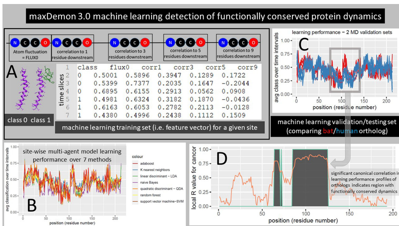
Figure 3. Detecting functionally conserved dynamics with the maxDemon 3.0 machine learning algorithm. (A) The MD simulation sets generated above are now the source of a pre-classified machine learning training set where class 0 and class 1 represent the binary functional states of the protein interaction (unbound vs. bound; Figure 1C). A feature vector is constructed comprising the atom fluctuations of any given amino acid (AA) site and its correlations to motions of downstream sites located 1, 3, 5, and 9 AA sites distant taken at every 50 frame intervals or 'time slices' in the MD simulations. This rich feature vector thus captures both the local energy on the protein backbone, as well as potential sequence-based information that coordinates specific motions with nearby AA sites. (B) A multi-agent classifier comprised of up to seven learning methods is individually deployed on each site and a learning performance profile across all sites on the protein is generated as the time average classification of the site-specific dynamics defined by the feature vector. Thus, successful learning of functional dynamic features will deviate from an average classification of 0.5 on the profile. (C) This learning profile is then modeled for two evolutionary homologs (e.g. human ACE2 bound to the recent emergent strain SARS-CoV-2 and bound to bat CoV-HKU4, a potential zoonotic precursor). (D) A local canonical correlation of the learning performance profiles from both homologs is taken over 20 adjacent AA sites from a sliding window moved across the protein. Significant correlation of the homologous learning profiles identifies regions (shown in gray) where the functional binding dynamics defined by the pre-classification is functionally conserved from the time of divergence of the viral homologs.
