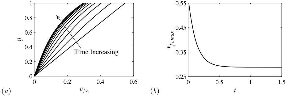
Fig. 11. The temporal evolution of the velocity field inside the layer of hydrogel with BC2 with parameters (\beta, \xi) = (0.5, 10) . (a) The variation of velocity along y-direction(vertical) of the ten different time t from 0.05 to 0.5 . (b) The evolution of the fluid velocity at the interface, also the maximum velocity in the hydrogel.
