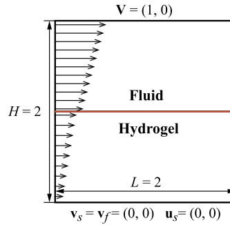
Fig. 7. The computational setup for a two-layer shear flow, with a layer of clear fluid flowing over a horizontal gel layer. The top boundary moves with a constant velocity V_x = 1 while the bottom is fixed. Periodic boundary conditions apply between the left and right boundaries.
