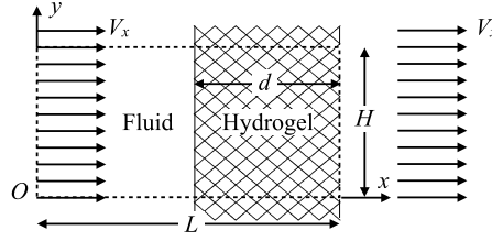
Fig. 2. Geometric setup of the 1D compression of a gel layer. We take the thickness of the gel layer to be the characteristic length L_0 such that d = 1 . The rectangular computational domain is indicated by the dashed line, with length L = 2 and height H = 1 .
