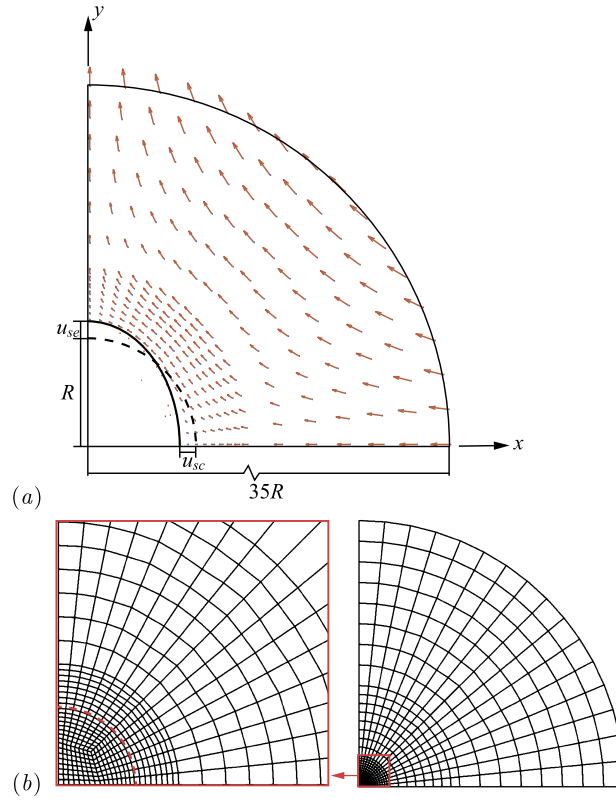
Fig. 12. (a) Planar elongation of the exterior fluids deforms a Darcy gel particle centered at the origin. The undeformed particle has a radius R = 1 , and the steady-state deformation of the particle is measured by the elongation at the north pole ( u_{se} ) and the compression at the equator ( u_{sc} ). (b) The mesh with minimum mesh size h_{min} = 0.06 inside the particle and maximum h_{max} = 3 along the exterior boundary, with a magnified view of the dense mesh around the particle. The red dash line is the initial location of the interface of the Darcy particle. (For interpretation of the colors in the figure(s), the reader is referred to the web version of this article.)
