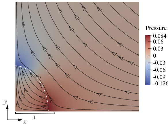
Fig. 13. Steady state streamlines and pressure contours around the Darcy gel particle, with dimensionless parameters Ca = 0.0375 , \xi = 400 , \eta = 0.0025 , \beta = 0.5 , \lambda_s = 1 , and \phi_{s0} = 0.5 . The white dash line delineates the steady-state interface between the gel particle and the pure fluid.
