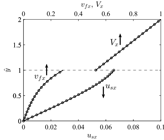
Fig. 8. The steady-state profiles in the two-layer shear flow, with boundary conditions BC2 on the fluid-gel interface and dimensionless parameters \mu_e = 1 , \lambda_s = 1 , \xi = 10 , \beta = 0.5 , \eta = 1 , Ca = 0.1 , and \phi_{s0} = 0.5 . The clear fluid has a linear profile V_x(\hat{y}) as expected, while inside the gel, nonlinear v_{fx}(\hat{y}) and u_{sx}(\hat{y}) profiles are entrained. The symbols denote the numerical results while the solid lines are theoretical solutions for a linearly elastic solid phase in the gel [42].
