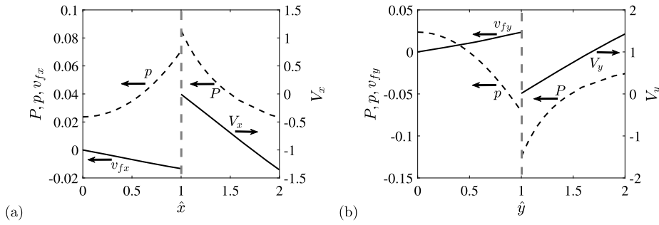
Fig. 14. (a) The pressure and fluid velocity profiles inside ( \hat{x} < 1 ) and outside the gel ( \hat{x} > 1 ) along the x -axis. Note the different velocity scales inside and outside the gel. (b) Similar profiles along the y -axis. In both plots, the gray dash line marks the location of interface.
