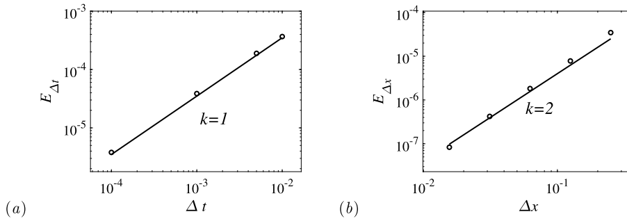
Fig. 6. (a) Convergence test with respect to the time step \Delta t . The error is for the interfacial value of solid fraction \phi_s|_{\tilde{x}=1} relative to the finest \Delta t = 2.5 \times 10^{-6} at t = 0.1 . The mesh size is fixed at \Delta x = 1/32 . The solid line indicates a slope of 1. (b) Convergence test with respect to the mesh size \Delta x . The error is computed from \phi_s|_{\tilde{x}=1} at t = 0.1 relative to the finest mesh \Delta x = 1/128 . The time step is fixed at \Delta t = 5 \times 10^{-6} . The solid line indicates a slope of 2. The parameters are the same as in Fig. 3 with \mu_e = 0 .
