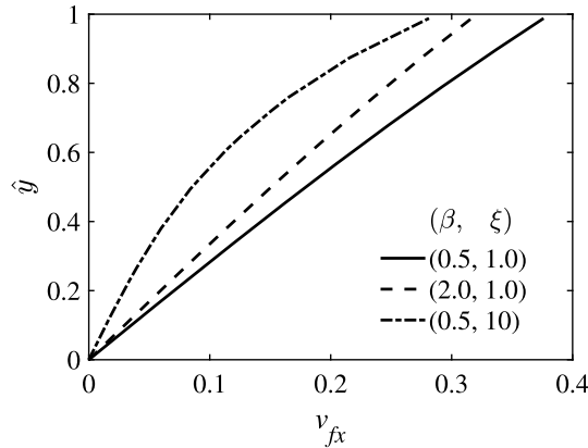
Fig. 9. Effects of the interfacial slip coefficient \beta and Darcy drag coefficient \xi on the shear velocity profile inside the gel layer. We have adopted BC2 on the fluid-gel interface. (\beta, \xi) = (0.5, 1.0) , (2.0, 1.0) , and (0.5, 10) from bottom to top. The other dimensionless parameters are the same as in Fig. 8.
