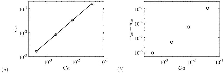
Fig. 15. (a) Gel particle deformation at the north pole u_{se} increases with the effective capillary number Ca . The other dimensionless parameters are fixed at the values of Fig. 13. The numerical results (symbols) are also compared with analytical solutions for the limit of small deformation (lines). (b) The difference of the two measures of deformation, u_{se} and u_{sc} .
