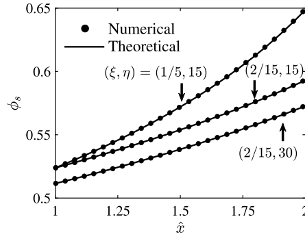
Fig. 5. Validation of the numerical solution of \phi_s by the analytical solution of Appendix B, for three sets of moderate parameters: (\xi, \eta) = (1/5, 15) , (2/15, 15) , and (2/15, 30) . The other parameters are the same as in Fig. 3 with \mu_e = 0 . The mesh size and the time step for this case are \Delta x = 1/8 and \Delta t = 0.01 , respectively.
