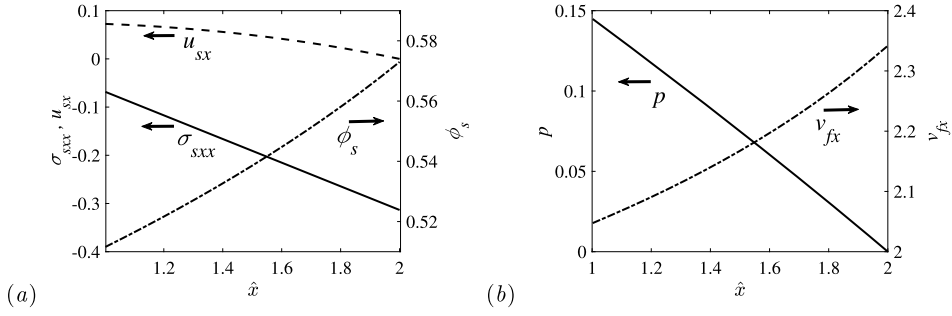
Fig. 4. Steady-state profiles for the Darcy-flow solution in the gel layer compressed by uniform flow. (a) The normal elastic stress \sigma_{sxx} , the displacement u_{sx} , and the solid fraction \phi_s along the \hat{x} -direction. (b) The pressure p and the fluid velocity v_{fx} along the \hat{x} -direction. The parameters are the same as in Fig. 3 with \mu_e = 0 .
