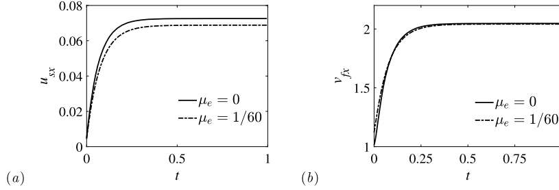
Fig. 3. The evolution of (a) the displacement u_{sx}|_{\hat{x}=1} and (b) the pore fluid velocity v_{fx}|_{\hat{x}=1} at the upstream interface \hat{x} = 1 . The solid curves represent the Darcy flow with effective viscosity \mu_e = 0 , and the dash-dot curves the Brinkman flow with \mu_e = 1/60 . The other dimensionless groups governing the problem are \lambda_s = 1 , \xi = 2/15 , \eta = 30 , Ca = 1 , and \phi_{s0} = 0.5 . The mesh size and the time step for this case are \Delta x = 1/8 and \Delta t = 0.01 , respectively.
