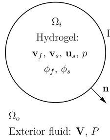
Fig. 1. A schematic of a particle of poroelastic gel in a Newtonian viscous fluid. The symbols are defined in the text.
