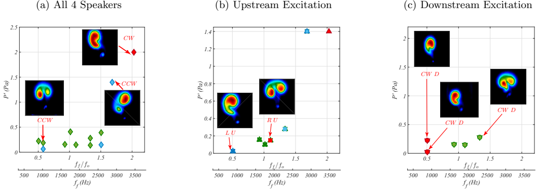
FIG. 10. Map of USL response, with representative mean cross-sectional jet PLIF images at x/D = 10.5 , to various speaker operational configurations: (a) All four speakers, (b) local upstream forcing, and (c) local downstream forcing. Symbols correspond to the legend in Fig. 7, where conditions are identified as LI (green), QP (blue), and NSR (red).
