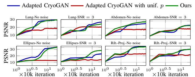
Fig. 12: Convergence results for the no noise and noisy (SNR = 3) experiments. The setting of the experiments are the same as the ones in Fig. 4-5. We compare UVTomo-GAN jointly optimizing for c and p (green) versus Adapted CryoGAN [32] (blue) and Adapted CryoGAN [32] with unif. p (red). Vertical axis shows the PSNR in dB and the horizontal axis is the training iteration number. The subplots in each row share the same vertical and horizontal axis.
