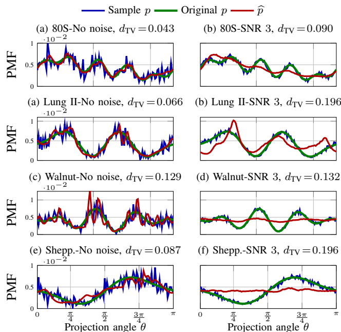
Fig. 11: Comparison between the original GT p (green) used to sample the viewing angles from, the empirical sample distribution of the viewing angles (blue) and the one estimated by our method \hat{p} (red). For more details on the computation of d_{TV} , refer to section VI-A and Fig. 7.
