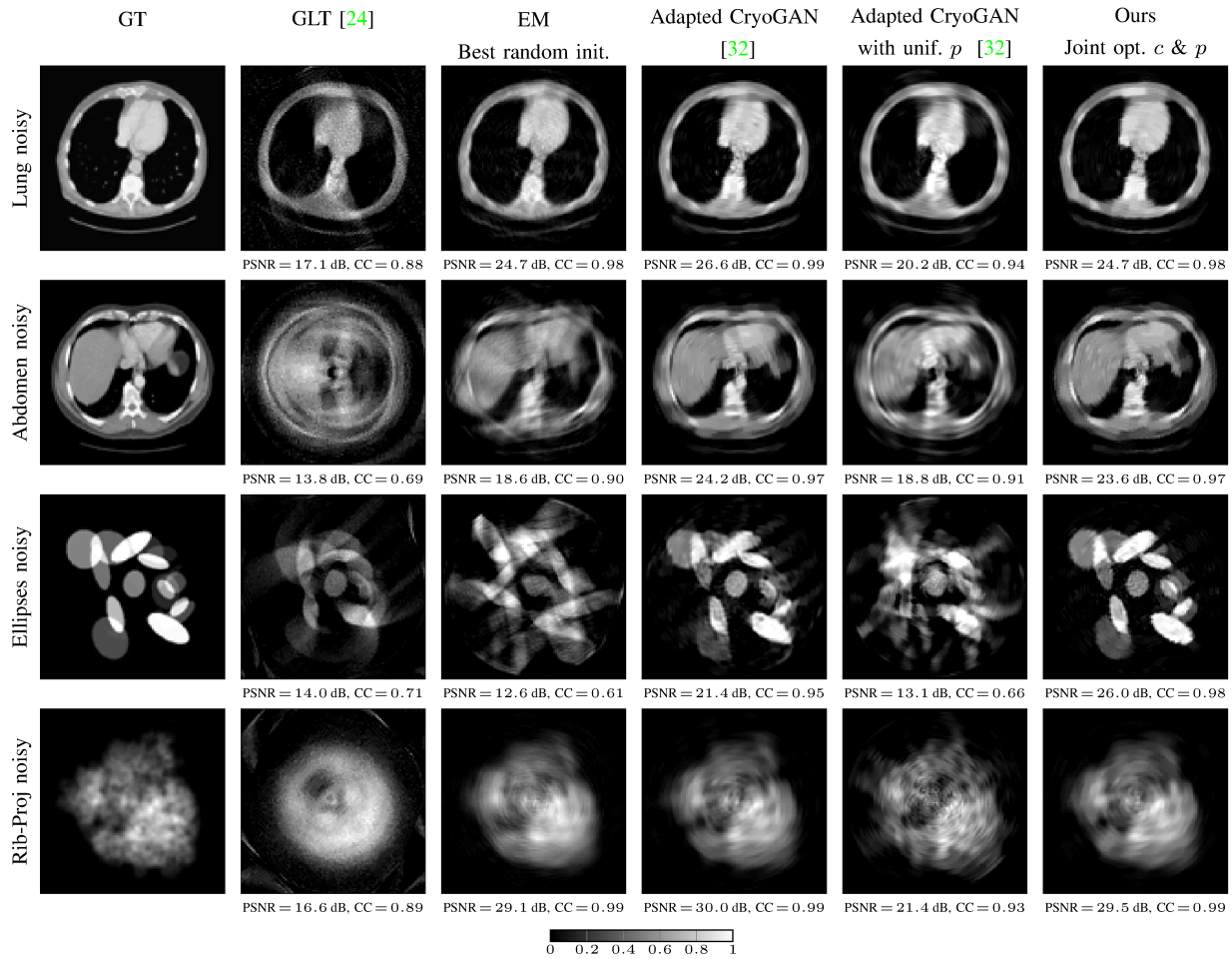
Fig. 5: Visual comparison of UVTomo-GAN with different baselines in noisy setting, i.e. \text{SNR} = 3 and L = 2 \times 10^4 . The description of the columns: 1) ground truth image (GT), 2) graph Laplacian tomography (GLT) [24], 3) EM with random initialization, 4) Adapted CryoGAN [32], 5) Adapted CryoGAN [32] with uniform p , 6) Ours, UVTomo-GAN with unknown p (jointly recovering c and p ). The PSNR and CC between the reconstructed images and the GT are provided.
