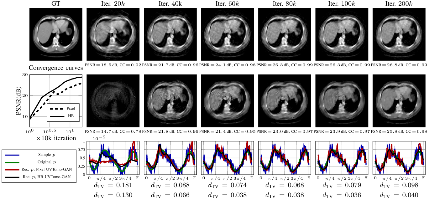
Fig. 8: Convergence of the reconstructed image and the viewing angle distribution throughout different iterations in a no noise setting for 1) UVTomo-GAN with HB image representation (first row), 2) UVTomo-GAN with pixel domain representation (second row). For each iteration, we report PSNR and CC of the reconstructed image and TV distance between the recovered p (red) and GT original p (green) from which the viewing angles are sampled, for both pixel and HB image representation (in second to last and last rows respectively). The sample estimation of p is plotted in blue. The evolution of PSNR throughout training iterations is plotted in second row, first subplot.
