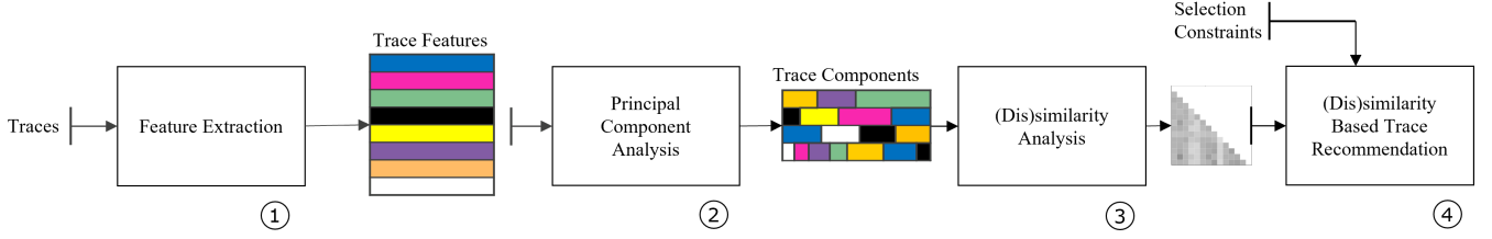
Figure 1: Workflow of IOTAP. It (1) extracts 253 features from each trace, (2) reduces its dimensionality through PCA (Principal Component Analysis), (3) computes the (dis)similarity between traces based on their distance in the PC dimension, and (4) sets forth a guideline for selecting traces.
