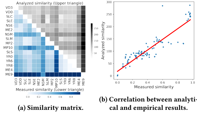
Figure 4: Figure 4a shows the similarity matrices between analytical (upper-right triangle in gray) and empirical (lower-left triangle in blue). Lighter shades indicate higher similarity, while the darker the more dissimilar. A greater degree of diagonal mirroring means a higher correlation between the analytical and empirical results. Figure 4b plots the correlation between analytical and empirical similarity. Each point represents a pairwise comparison between two distinct traces in Table 5. The correlation coefficient is 0.92.
