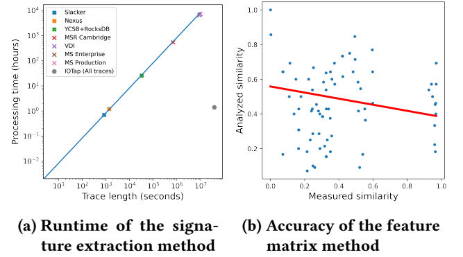
Figure 5: Performance and accuracy of prior methods. Figure 5a plots the trace processing time for the signature extraction method [4]. The measured processing time (in bold \times ) for the Slacker, Nexus, and YCSB+RocksDB traces are 0.6, 1, and 24 hours, respectively. On the other hand, IOTAP only takes 1.4 hours to extract features from all 3258 traces together. Figure 5b shows the correlation between the empirically measured similarity and the analytical similarity using the feature matrix method [20]. The two do not correlate well, with a correlation coefficient of -0.19.
