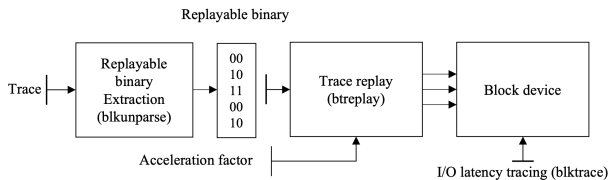
Figure 3: Replaying and measuring latencies of I/O traces for empirical validation: (1) blkunparse converts the block I/O in text format into a replayable binary format, (2) btoreplay replays the trace binary with an acceleration factor on a test device, (3) and blktrace measures the latencies.
