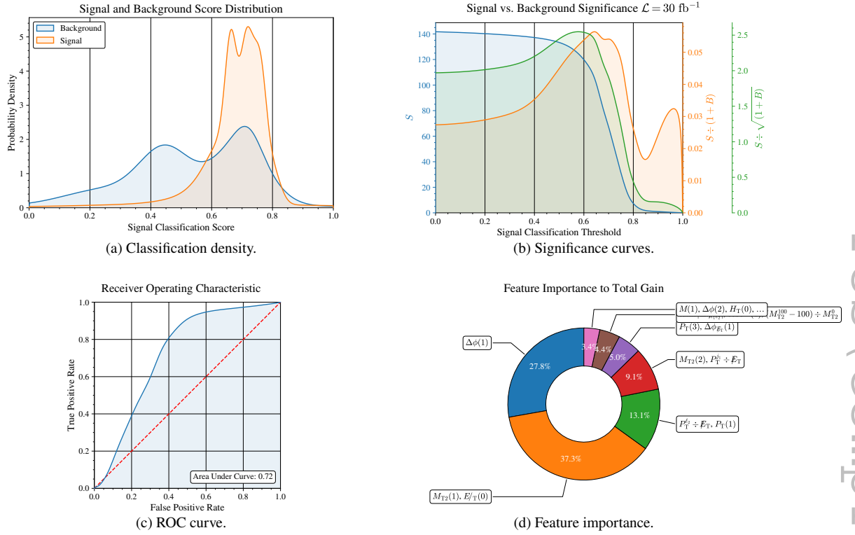
Figure 3: Joint training.
