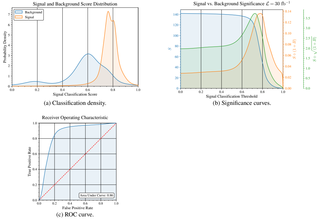
Figure 4: Ensemble training.
