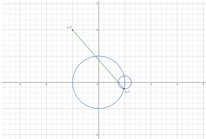
Figure 1: An example scenario for z_1 and z_0 .
