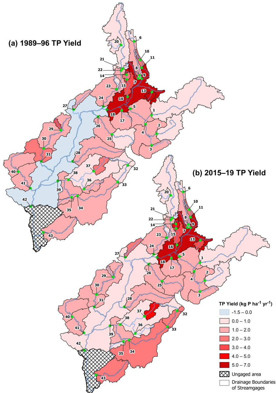
FIGURE 2. Incremental total phosphorus (TP) yields in kilograms phosphorus per hectare-year ( \text{kg P/ha/year} ) in the Illinois River Basin during (a) 1989–1996, and (b) 2015–2019 (see Table 1 for monitoring location names).
