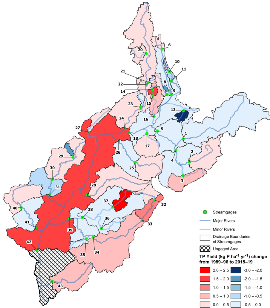
FIGURE 3. Changes in incremental TP yields in kilograms phosphorus per hectare-year (kg P/ha/year) from 1989–1996 to 2015–2019. See Table 1 for monitoring location names.
