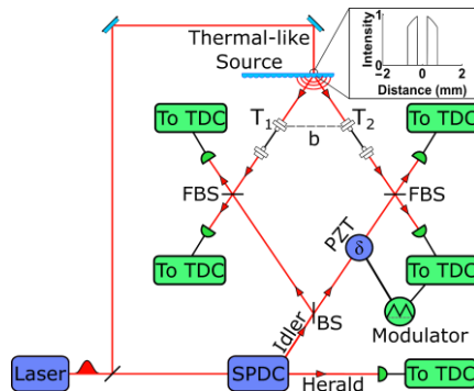
Fig. 1: A pulsed laser pumps both an SPDC and a thermal-like source which are used for laboratory long-baseline imaging as proposed by GJC.
