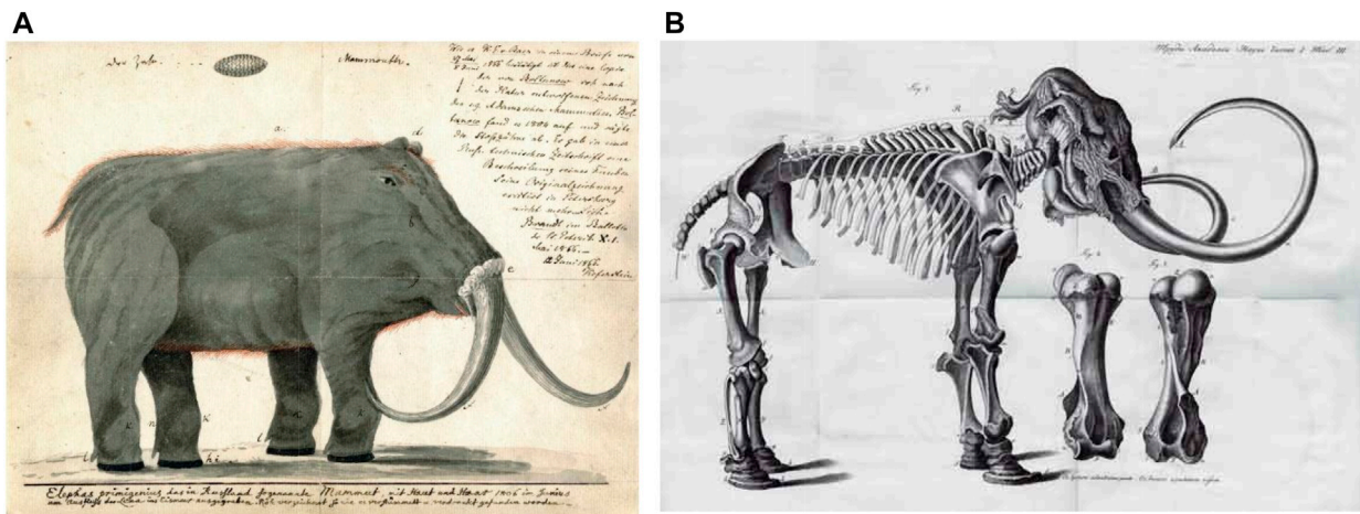
FIGURE 2 | (A) —The world's first reconstruction drawing of a mummified carcass of the so-called “Adams or Lena Mammoth” based on the original sketch by Roman Boltunov (in the Ethnological Collection of the University of Göttingen); (B) —Wilhelm Gottlieb Tilesius’ etching of the Adams mammoth skeleton (now on display in the Museum of Zoology, Sankt-Peterburg).
