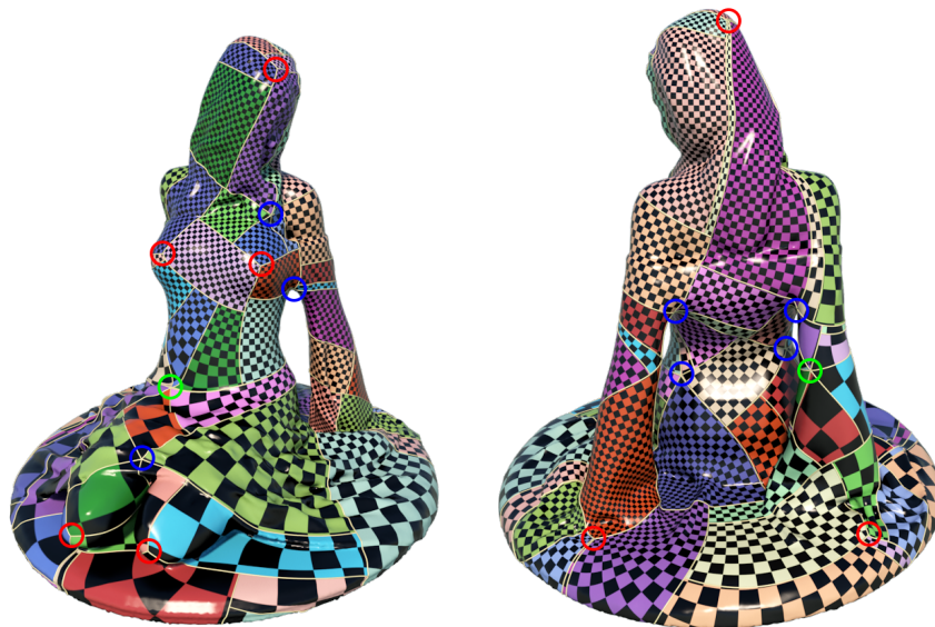
Figure 9: Singularities and T-Mesh of the Loveme model.
