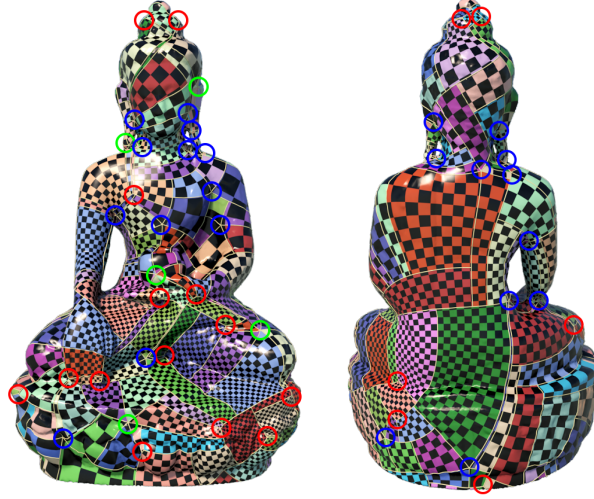
Figure 5: The singularities of the Buddha surface. The valences of the singularities are 3 (red), 5 (blue) and 6 (green) respectively.
