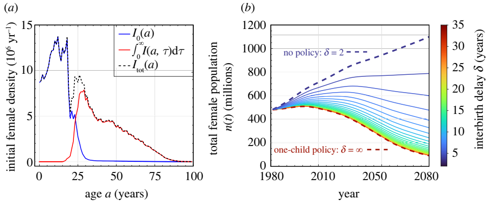
Figure 4. Evolution of the population for different delays. (a) Initial female subpopulation distributions in 1981 China (calculated from Population Census Office under the State Council [20]). (b) Evolution of the total female population n(t) for different imposed delays between births. These results are determined using the birth and death rates in figure 1 and the initial populations shown in (a). A relatively small delay between births (for example, \delta \sim 4 years) has a significant impact on the evolution of n(t) .
