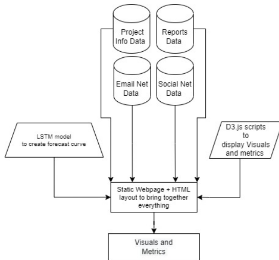
Figure 1: The APEX pipeline
