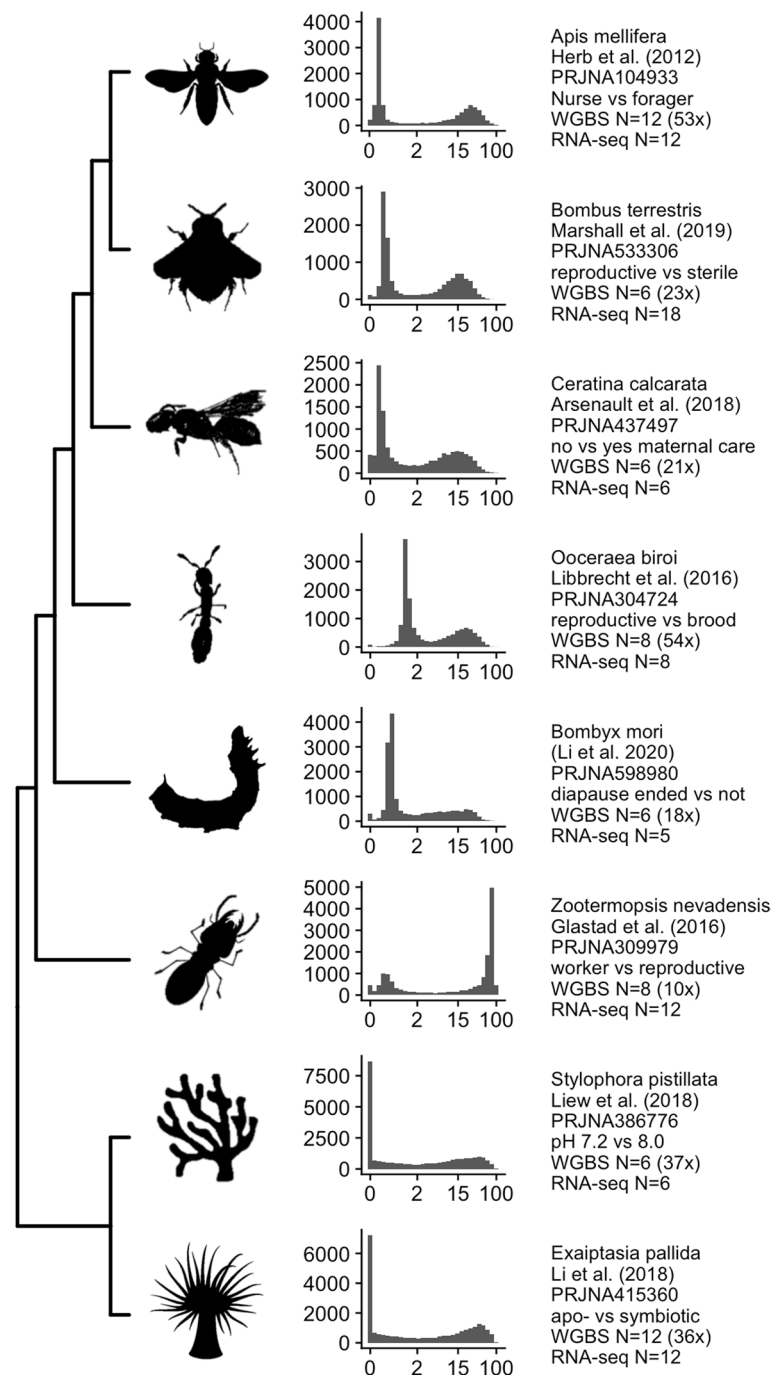
Fig. 1 Overview of species covered by previously published datasets and the distribution of GBM levels in each. X-axes for histograms show percent methylation (summed across all CpG sites within the gene and averaged across all samples from each study) on the \log_2 scale. The Y-axes show the counts of genes. Text reports the species, reference, NCBI Bioproject accession, the treatment groups compared here, the Whole Genome Bisulfite sample size (with mean genomic coverage), and the RNA-seq sample size for each study
