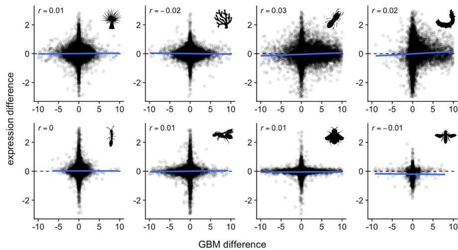
Fig. 4 Changes in GBM and transcription between phenotypic conditions showed no clear relationship. X axes indicate differential GBM estimated using MethylKit. Y axes indicate differential transcription estimated using DESeq2. Both axes are on the \log_2 scale. Correlation coefficient is given in the upper left of each plot. Contrasts used to compute differential GBM and transcription are given in Fig. 1
