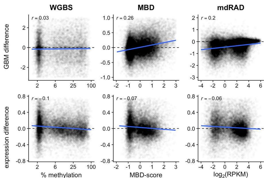
Fig. 5 Class-level shifts in GBM and transcription in A. millepora . X axes show baseline GBM level averaged across all samples. Y axes shows differential GBM between polyp types (top panels) and differential transcription between polyp types (bottom panels). Top panels: Differential GBM between polyp types was linked with baseline GBM level for the MBD-seq and mRAD datasets, but not for WGBS. Bottom panels: For all three methylation datasets, the low GBM class of genes was somewhat upregulated in axial compared to radial polyps, and the high GBM class was somewhat downregulated
