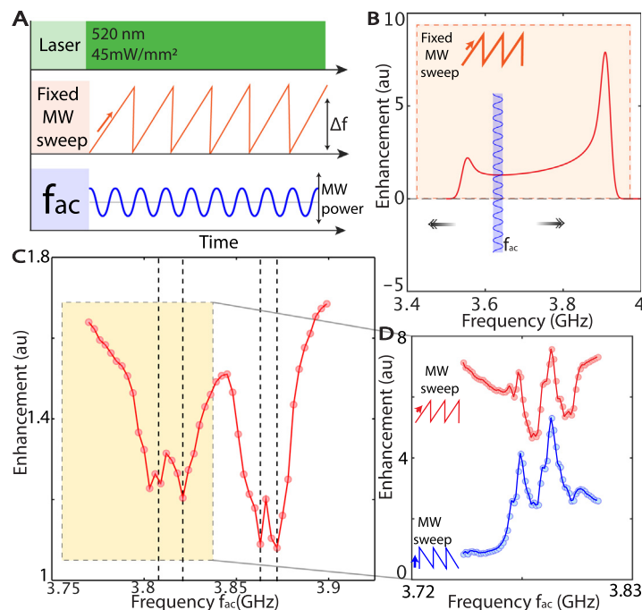
Fig. 4. “Hole burning” DNP experiments to unravel homogeneously broadened NV center spectra. (A) Protocol consists of MW chirps applied over a wide (fixed) bandwidth \Delta f (orange) and a single MW tone at frequency f_{ac} (blue). (B) Principle: Consider an NV ESR spectrum (red), and applied MW chirp over the wide bandwidth (orange). Now, for the NV centers resonant with the tone f_{ac} (blue), there is a saturation of the NV population, and hence loss of ^{13}\text{C} hyperpolarization transferred via the swept MWs. Upon varying tone frequency f_{ac} , this manifests as a “hole” in the obtained DNP spectrum at NV center resonance, therefore unraveling with high contrast the NV ESR spectrum. (C) hole-burned DNP carried out on a single crystal sample with varying f_{ac} reveals the four underlying NV center orientations (dashed lines) constituting an originally broad DNP profile. (D) Zoom in to the two NV families on the left (shaded in C) via hole-burning DNP, with chirped MWs applied with low-to-high or high-to-low frequency. Hole burned spectra manifest with opposite sign than those in Fig. 3.
