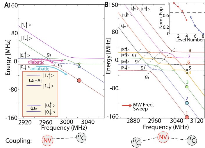
Fig. 2. DNP mechanism. (A) Landau-Zener anticrossings in the rotating frame with assumed Rabi frequency \Omega_c , and A_{\perp} = A_{\parallel} . We assume applied low-to-high frequency sweeps, starting with an initial unpolarized nuclear state in the m_s = 0 manifold. Inset shows lab frame energy levels for an NV- ^{13}\text{C} system, restricted to the m_s = \{0, +1\} manifolds. We assume to work at low-fields wherein nuclear Larmor frequency \omega_L < A_{\parallel} . Dashed lines indicate the crossings assuming A_{\perp} = 0 . The two LZ energy gaps \{g_1, g_2\} conditioning the nuclear spin states |\downarrow\rangle and |\uparrow\rangle , are large and small respectively, leading to adiabatic and diabatic transitions upon traversals through the LAC system (blue and red lines). This leads to population bias in the lower branch (balls show populations) and ^{13}\text{C} hyperpolarization in nuclear state |\downarrow\rangle upon NV repolarization. (B) System with two ^{13}\text{C} nuclei coupled to an NV center. In this toy model, we assume effective nuclear frequencies for the two nuclei \omega_j^{(0,1)} in the m_s = \{0, 1\} manifold such that \omega_j^{(0)} = 2j^p ; \omega_j^{(1)} = 5j^p , where p = 1.1 . There are multiple LZ anticrossings, and a hierarchy of energy gaps ( g_1 - g_4 ) are successively traversed upon a low-to-high frequency sweep. Time evolution starting with an nuclear unpolarized state leads to system bias and hyperpolarization in the lower two energy levels (inset).
