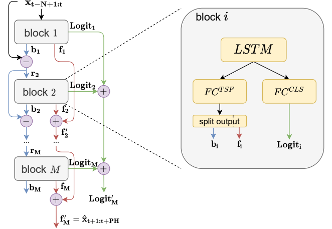
Fig. 1. Architecture of the proposed multitask learning system. Block structure of N-BEATS (left). A classification branch is added to each block (right).
