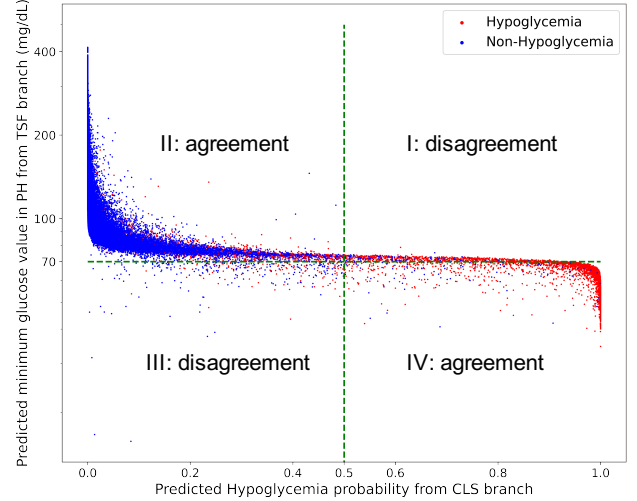
Fig. 3. Predictions from the two branches of the multitask learning model. Red points represent instances of HG.
