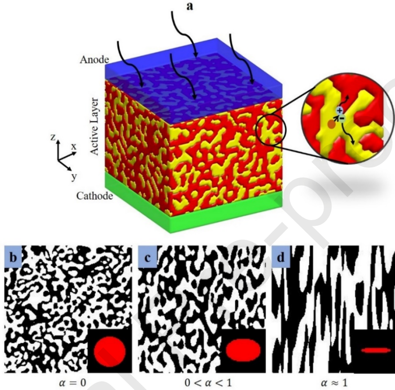
Fig. 5. (a) Schematic representation of OPVCs. Inset shows excitons (orange) dissociating into protons (blue) and electrons (green), which travel to the anode and cathode, respectively. (b–d) Quantifying anisotropy for microstructures with elliptical SDF using anisotropy index \alpha .
