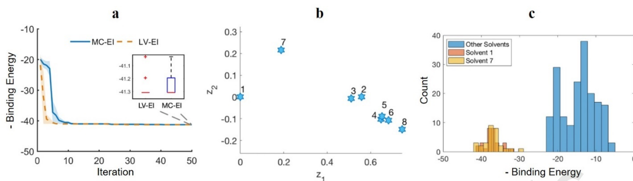
Fig. 11. (a) Comparing the convergence BO with the EI acquisition function for MC-EI and the LV-EI GP. (b) Latent space for the “solvent type” categorical variable with eight levels. (c) Distribution of binding energy categorized by “solvent type.”
