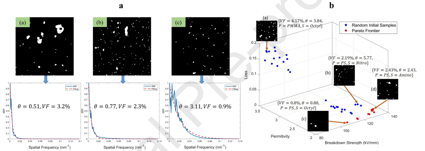
Fig. 10. Concurrent composition and microstructure design for nanocomposites. (a) SDF characterizes nanoparticle dispersion using parameter \theta and nanoparticles loading using the VF. (b) Multicriteria mixed-variable BO using LVGP identifies the Pareto frontier displaying significant improvement with respect to randomly selected initialization samples ( P stands for polymer type; S stands for type of surface treatment. PMMA: polymethyl methacrylate; PS: polystyrene).
