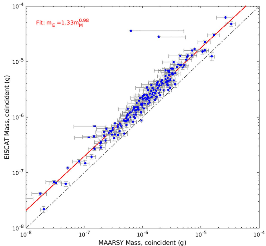
Figure 6. Masses estimated using EISCAT versus MAARSY data, with 1\sigma error bars. The black dashed line represents exact equality. The red line represents a linear fit in log-log space, neglecting outliers. The fit shows that there is a strong linear correlation between the two estimates, but that the EISCAT estimates are on average a factor of 1.33 greater than the MAARSY estimates.
