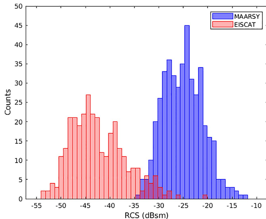
Figure 1. Histograms of the median radar cross section for each radar profile for MAARSY (blue) and EISCAT (red).
