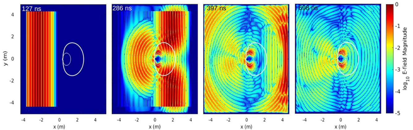
Figure 3. Snapshots from an finite difference time domain simulation. The simulated radar pulse enters the box from the left (panel 1) and interacts with the meteor plasma, represented by the white contour lines (panel 2). The thin inner line represents the overdense area, or the region in which the plasma frequency \omega_p is greater than the transmitted frequency \omega ( \omega_p \geq \omega ). The thick outer line represents the region in which the plasma frequency has dropped to a factor of e less than the transmitted frequency, ( \omega_p \geq \omega/e ). Some portion of the pulse reflects from the plasma (panel 3), leaving small-scale perturbations behind (panel 4).
