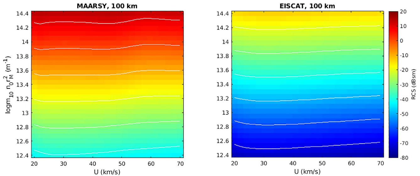
Figure 5. MAARSY (left) and EISCAT (right) lookup tables at 100 km. Contours are drawn at intervals of 10 dB.
