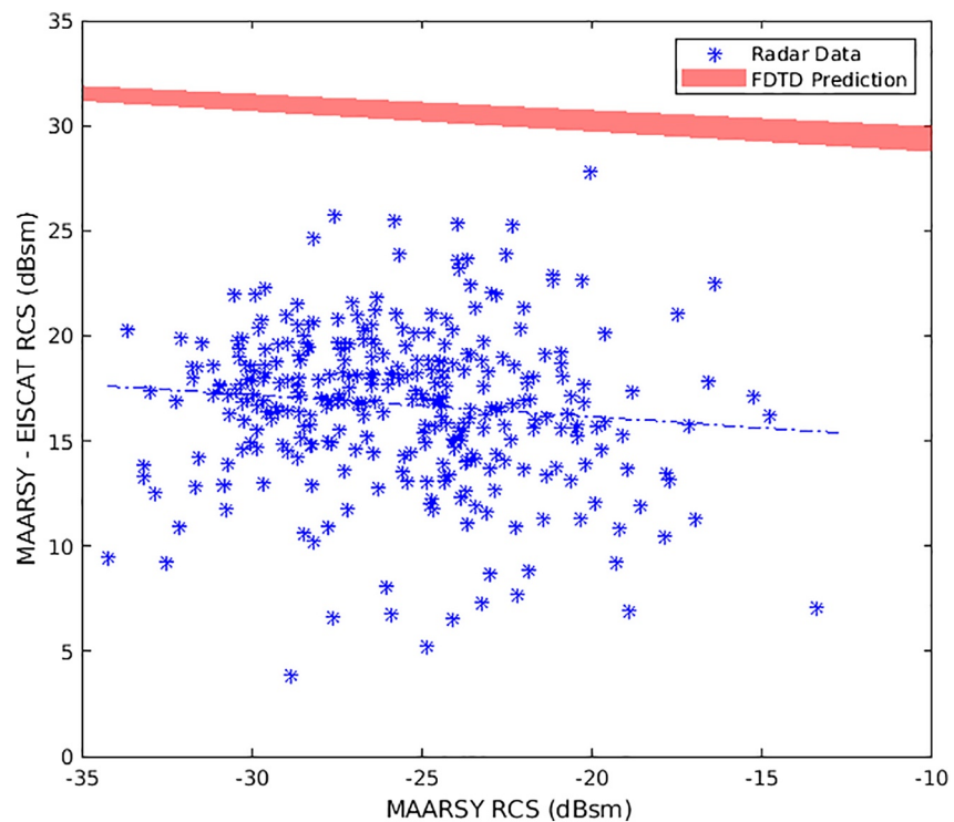
Figure 8. Radar cross section difference between MAARSY and EISCAT observations, as predicted by the finite difference time domain model (red) and in the data (blue). A linear fit to the radar data is shown by the blue dashed line.
