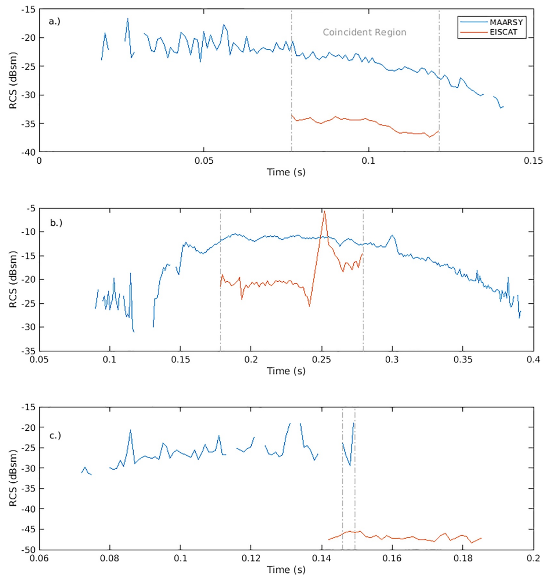
Figure 2. Example radar cross section profiles. The coincident region, where both radar observe the meteor at the same time, is marked by dashed lines. Many profiles are smooth (a), but some have sudden large spikes or troughs (b), significant gaps in the observation, or are only observed coincidentally at a few points (c).
