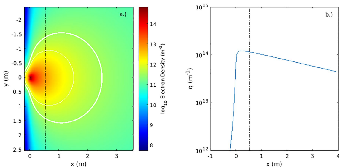
Figure 4. Example of the Dimant-Oppenheim head plasma distribution, for a meteor at 100 km traveling at 60 km/s (a.). Contours are the same as in Figure 3. The location in the tail at which the line density q is calculated is shown by the black dashed line. The value of q at each grid location is shown on the right (b.).
