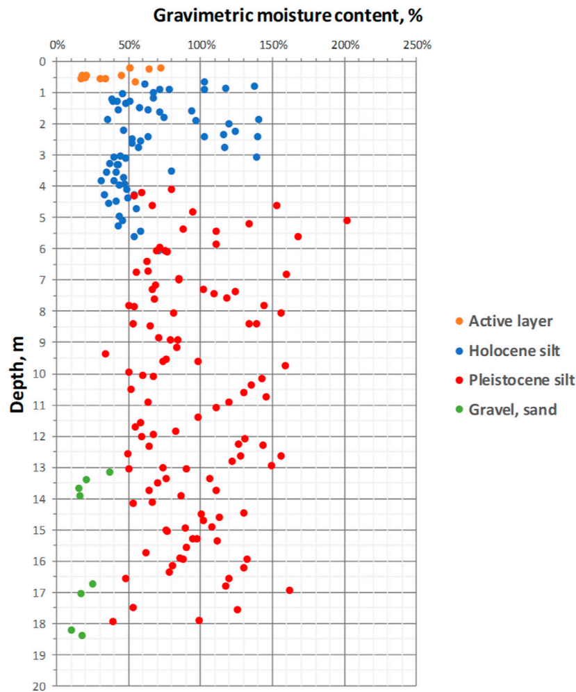
FIGURE 5 | Gravimetric moisture contents of sediments with depth, based on the drilling data (Boreholes F1, F2, F3, F4, F12, and F16). Average values: Active layer— 39.7 \pm 19.3\% ( n = 12 ); Holocene silt (including the intermediate layer)— 65.4 \pm 31.0\% ( n = 64 ); Pleistocene silt— 94.0 \pm 34.4\% ( n = 111 ); Gravel and gravelly sand— 19.9 \pm 8.0\% ( n = 8 ).
