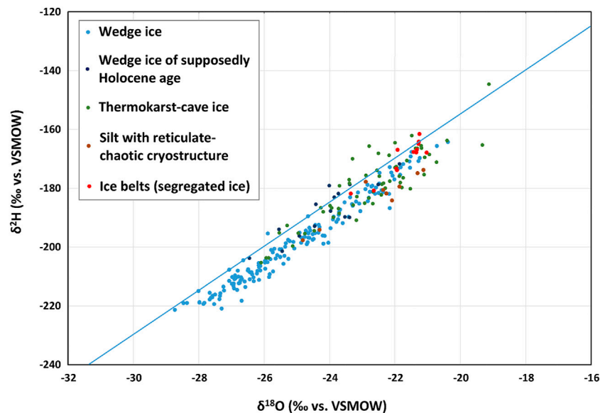
FIGURE 11 | \delta^{18}\text{O} – \delta^2\text{H} diagram for different types of ground ice in the CRREL Permafrost Tunnel. Blue line represents the Global Meteoric Water Line (GMWL).
