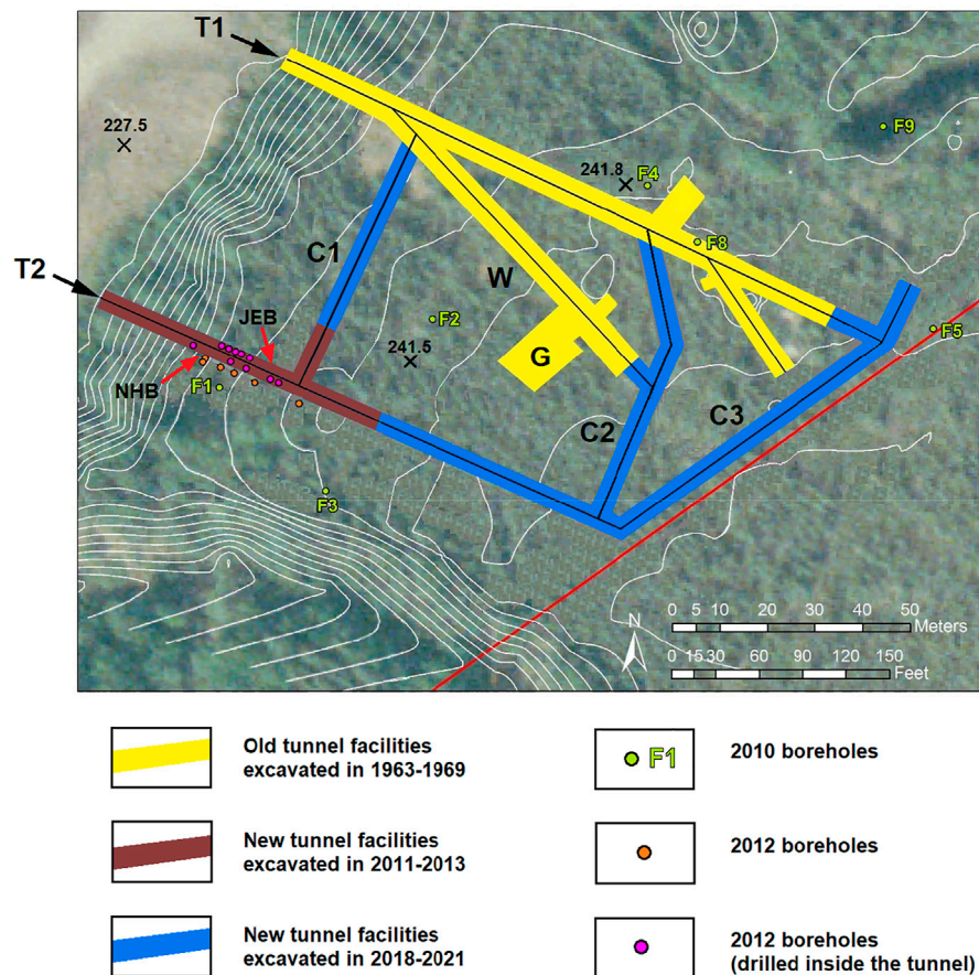
FIGURE 2 | Plan view of the CRREL Permafrost Tunnel facilities, including old (northern adit, T1) and new (southern adit, T2) Tunnels, inclined winze (W), gravel room (G), crosscuts that connect old and new Tunnels (C1, C2, and C3), and boreholes. Locations of NHB and JEB sections are marked with red arrows. Contour lines have 1 m intervals. Modified from Bjella and Sturm (2012).
