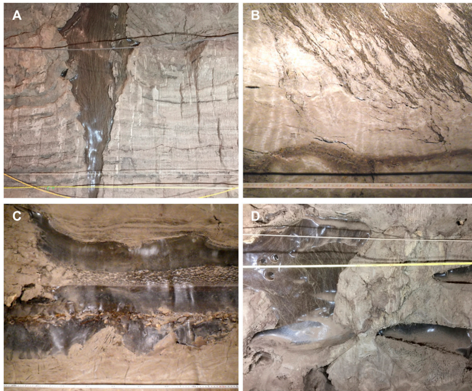
FIGURE 8 | Massive-ice bodies exposed in the new Permafrost Tunnel. For locations, see Figures 6, 7, 10 . (A) Syngenetic ice wedge. Left wall of Crosscut #1 of the new Tunnel (C1), distance 9.4–13.9 m, elevation 228.8–231.6 m. (B) Ice wedge surrounded by individual ice veins forming composite (ice/silt) wedge; note a dark-brown layer of buried peat. Right wall of the main adit of the new Tunnel (T2), distance 32.8–33.4 m, elevation 229.0–229.5 m. (C) Thermokarst-cave ice. Horizontal stratification and suspended wood fragments indicate several stages of water accumulation and thermokarst-cave ice aggradation in the underground cavity. Right wall of the main adit of the new Tunnel (T2), distance 38.9–39.9 m, elevation 229.0–229.9 m. (D) Underground erosional channels filled with thermokarst-cave ice underlain by silt with reticulate-chaotic cryostructure. The channels started developing along ice wedges but eventually expanded and affected enclosing sediments. Left wall of Crosscut #1 of the new Tunnel (C1), distance 27.0–28.6 m, elevation 228.2–229.4 m.
