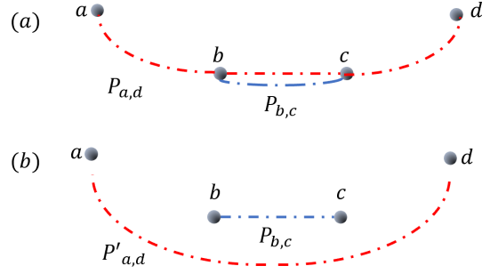
Fig. 4: Illustrating the simple greedy scheme, and the GG Algorithm with Update and Append options. (a) Two SLs (a, d) and (b, c) shown with associated (shortest) paths P_{ad} and P_{bc} respectively; these paths are not disjoint. (b) New non-shortest path P'_{ad} for (a, d) which doesn't intersect with (b, c) 's associated path P_{bc} . If SL (b, c) (with associated path P_{bc} ) is first/already chosen as an SL in the solution, then a simple greedy algorithm will not consider (a, d) as a super-link since its associated path P_{ad} intersects with P_{bc} . Instead, the GG Algorithm considers including super-link (a, d) in the solution via two options: (i) Update : Remove (b, c) , and add (a, d) with associated (shortest) path P_{ad} , or (ii) Append : Add (a, d) with associated path P'_{ad} .
