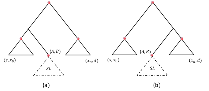
Fig. 2: Two possible swapping trees to generate EP over (s, d) pair using a super-link (A, B) .
