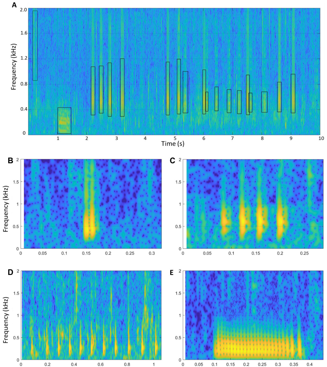
Fig. 2. (A) Example spectrogram with bounding boxes around fish sounds and 4 commonly seen call types: (B) double pulse between ~0.2–1 kHz, (C) multipulsed between ~0.2–1 kHz, (D) rapid pulse between ~0.1–0.5 kHz, and (E) low-frequency burst pulse call between ~0–0.5 kHz
