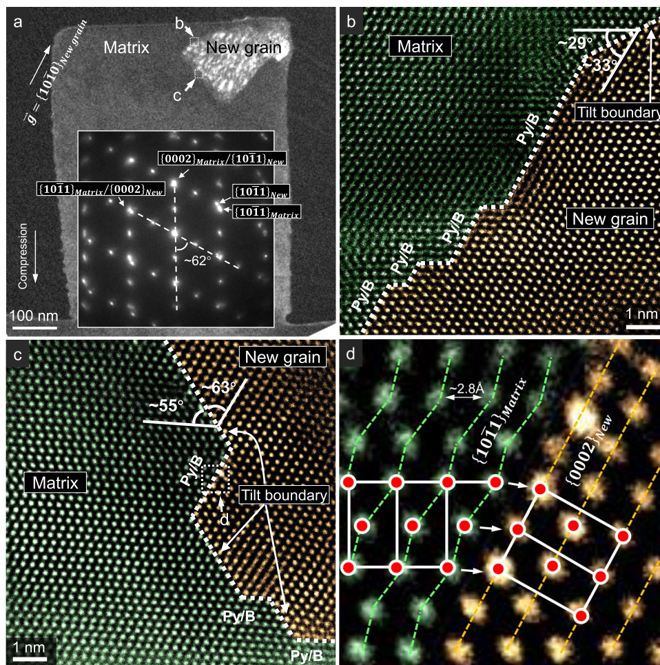
Fig. 4 Atomic structure of the grain boundaries of a new grain formed during c-axis compression. a TEM dark-field image showing the morphology of this new grain. The inset selected area diffraction patterns indicate the orientation relationship of \{10\bar{1}1\}_{\text{Matrix}} \parallel \{0002\}_{\text{New}} and \{0002\}_{\text{Matrix}} \parallel \{10\bar{1}1\}_{\text{New}} . b, c Py/B interfaces and basal plane tilt boundaries, acquired from the places marked by the white dashed frames labeled by “b” and “c” in a , respectively. d Fine structure of the Py/B interface, acquired from the place marked by the white dashed frame labeled by “d” in c . The green and orange dashed lines are the traces of corrugated \{10\bar{1}1\} and flat \{0002\} planes, respectively. The HCP unit cells of the matrix and the new grain are highlighted by the white lines and red circles. The zone axis is \sim(2\bar{1}10) .
