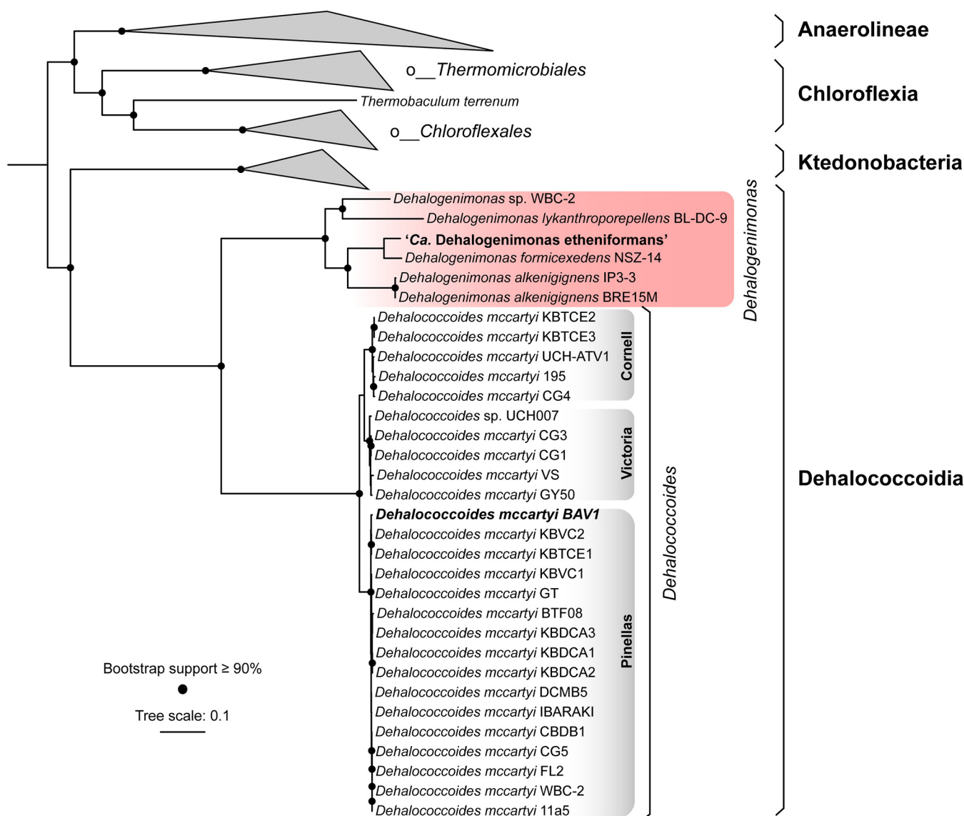
FIG 1 Phylogeny of Dehalococcidia . The tree was constructed using an alignment of 120 conserved single-copy genes obtained using the GTDB-Tk and the maximum-likelihood algorithm. Bootstrap values \geq 90\% are shown. Scale bar represents 0.1 substitutions per site. Classes within the Chloroflexi phylum are labeled on the right in bold, and clades Thermomicrobiales , Chloroflexales , Dehalogenimonas , and Dehalococcoides are shown in italics. Labels correspond to the taxonomy proposed by the GTDB.
