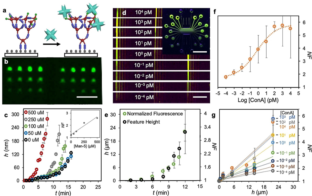
Figure 3. a) ConA binding to the Man-5-containing GTGFRP brushes. b) Fluorescence microscopy of FITC-ConA bound to Man-5-containing GTGFRP brushes. Scale bar is 100 \mu\text{m} . c) Effect of varying [Man-5] on GTGFRP polymer growth rate ([EGDMA] = 1300 mM; [TPO] = 1 mM; light intensity = 1.16 \text{ mW mm}^{-2} ; [PETT] = 100 mm). The inset shows the effect of varying [Man-5] on fluorescence with polymer brushes with heights of 110 \pm 10 \text{ nm} . d) Fluorescence image of Man-5-containing GTGFRP brushes of varying heights patterned into vertical lines after exposure to FITC-ConA. Scale bar is 300 \mu\text{m} . Inset is a fluorescence image of the incubation chip containing FITC-ConA solutions at 9 different concentrations. Scale bar is 5 mm. e) The height and NF of the vertical line pattern of Man-5-containing GTGFRP glycopolymers from the channel with 0.1 pM FITC-ConA. f) Relationship between [ConA] and NF for feature heights of 22 \pm 3.8 \mu\text{m} . g) Relationship between height Man-5 and NF of Man-5-containing GTGFRP polymers upon exposure to solutions with different [FITC-ConA]. Heights are reported as the average of 3 features of the same exposure time, and all error bars are reported as one standard deviation from the mean.
