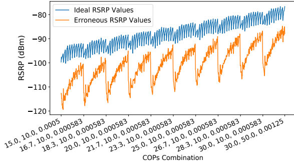
Figure 2: The COP-KPI database trends with the ideal and non ideal cases.
