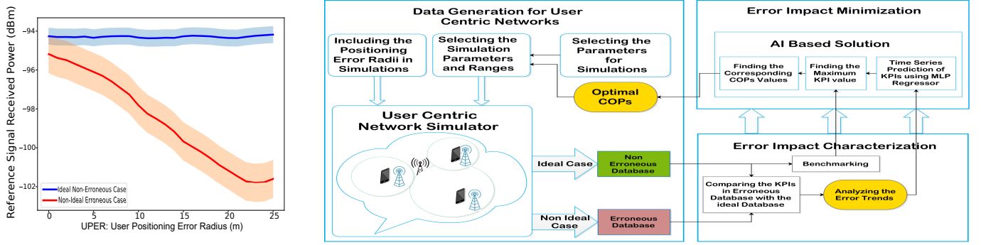
Figure 1: (a). The increasing fall in RSRP with respect to user positioning error radius (UPER), (b). The framework for error impact characterization and its minimization using the TS based modeling in UC-RAN.
