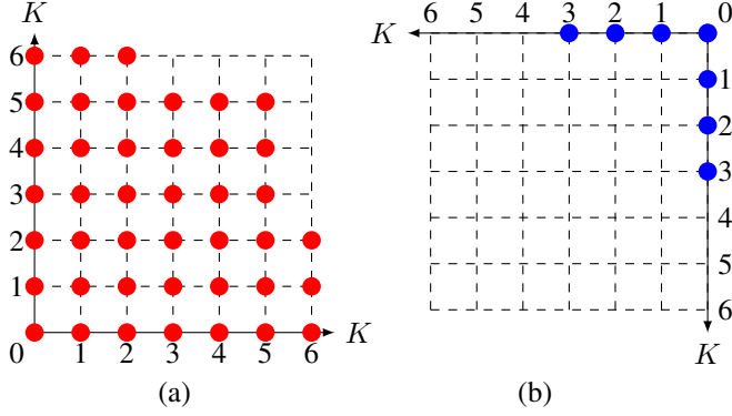
Fig. 3: The code \text{ARM2}(K^2, 2) in Example 3.3 with K = \mathbb{F}_7 is generated by the vectors \text{ev}_{K^2}(\mathbf{M}) , where \mathbf{M} is a monomial whose exponent corresponds to a point in (a). The dual \text{ARM2}(K^2, 2)^\perp is generated by the vectors \text{ev}_{K^2}(\mathbf{M}) , where \mathbf{M} is a monomial whose exponent corresponds to a point in (b).
