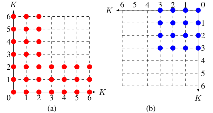
Fig. 1: The \text{ARM1}(K^2, 2) code in Example 2.4 with K = \mathbb{F}_7 is generated by the vectors \text{ev}_{K^2}(\mathbf{M}) , where \mathbf{M} is a monomial whose exponent corresponds to a point in (a). \text{ARM1}(K^2, 2)^\perp is generated by the vectors \text{ev}_{K^2}(\mathbf{M}) , where \mathbf{M} is a monomial whose exponent corresponds to a point in (b).
