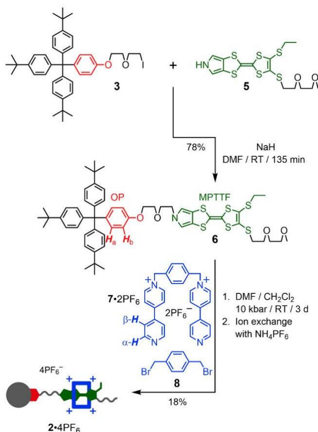
Scheme 3 Synthesis of the dumbbell 6 and the [2]rotaxane 2 •4PF 6 .
