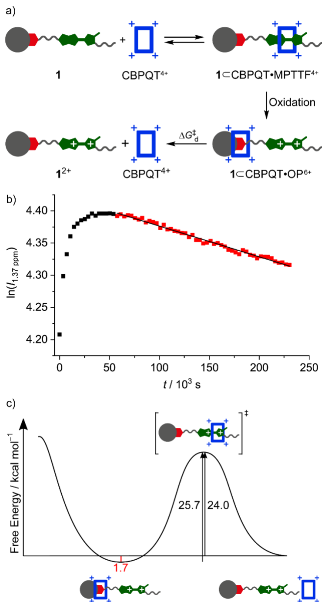
Fig. 8 A cartoon representation illustrating the oxidation process of 1 ⊂CBPQT•MPTTF 4+ leading initially to the formation of 1 ⊂CBPQT•OP 6+ followed by the slow production of uncomplexed semidumbbell 1 2+ and CBPQT 4+ . b) Plot of \ln I against t at 294 K for the deslipping of CBPQT 4+ from 1 ⊂CBPQT•OP 6+ by using the integral ( I ) at 1.37 ppm as the probe. The red data points have been fitted by the best straight line, giving a correlation coefficient of 0.989, indicating that first order kinetic are in operation. The slope of the line gives the rate constant k_d , according to relationship \ln I = -k_d t . c) Energy diagram for the deslipping of CBPQT 4+ from the OP moiety across the MPTTF 2+ unit in the [2]pseudorotaxane 1 ⊂CBPQT•OP 6+ in CD 3 CN at 298 K.
