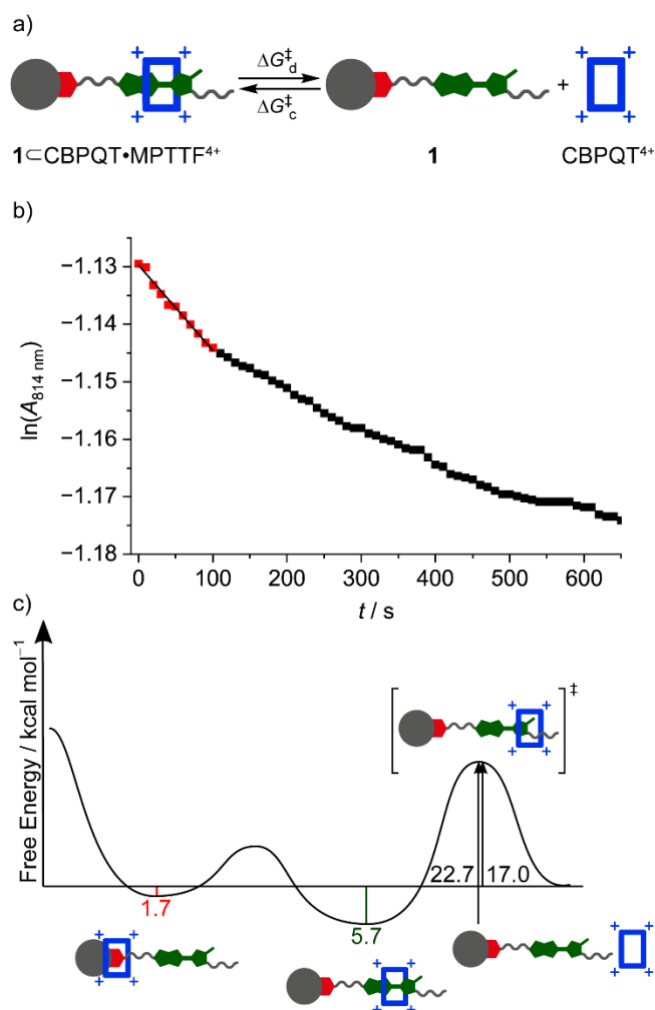
Fig. 6 a) A cartoon representation illustrating the decomplexation/complexation between the [2]pseudorotaxane 1\subset\text{CBPQT}\cdot\text{MPTTF}^{4+} and the uncomplexed species 1 and \text{CBPQT}^{4+} . b) Plot of \ln A against t at 298 K for the decomplexation (d) of \text{CBPQT}^{4+} from 1\subset\text{CBPQT}\cdot\text{MPTTF}^{4+} by using the absorption ( A ) at 814 nm as the probe. The data points were collected in the early stage of the experiments where the complexation (c) process is not yet occurring to any significant extent and the red data points have been fitted by the best straight line, giving a correlation coefficient of 0.98, indicating that first order kinetic is in operation. The slope of the line gives the rate constant k_d , according to relationship \ln A = -k_d t . c) Energy diagram for the movement of \text{CBPQT}^{4+} away from the MPTTF unit in the [2]pseudorotaxane 1\subset\text{CBPQT}\cdot\text{MPTTF}^{4+} in MeCN at 298 K.
