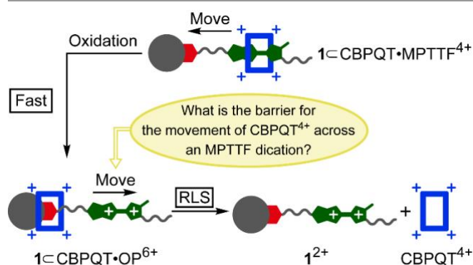
Scheme 1 Oxidation of the monopyrrolotetrathiafulvalene (MPTTF) unit in 1 CBPQT•MPTTF 4+ to produce 1 CBPQT•OP 6+ , which subsequently deslips in a slow and rate-limiting step (RLS) producing 1 2+ and CBPQT 4+ .
