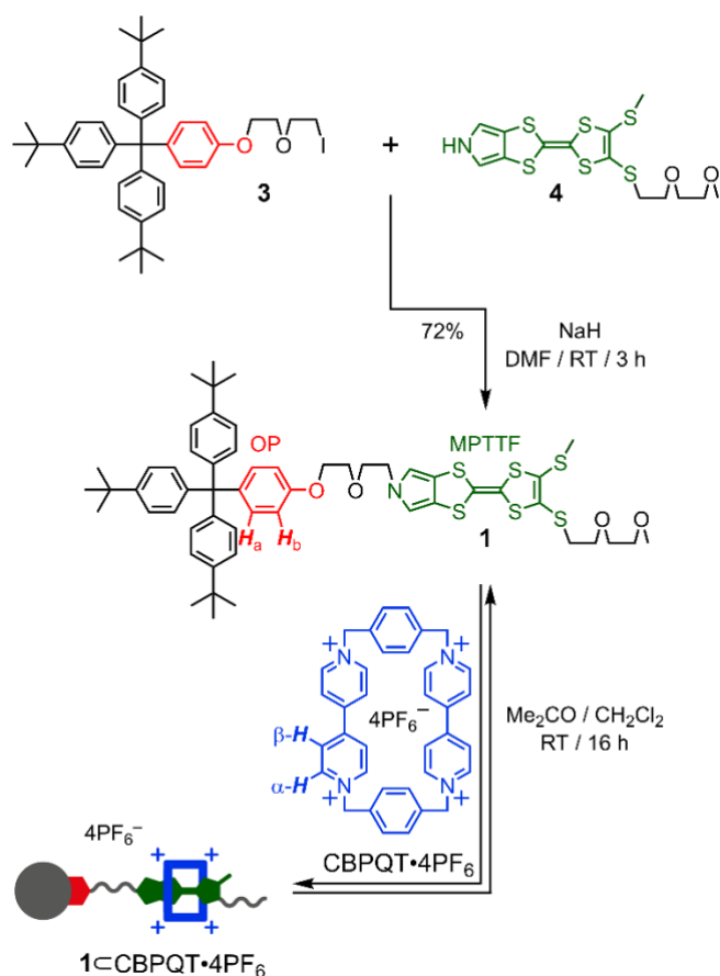
Scheme 2 Synthesis of the semidumbbell 1 and self-assembly of the [2]pseudorotaxane 1 ⊂CBPQT•4PF 6 .
