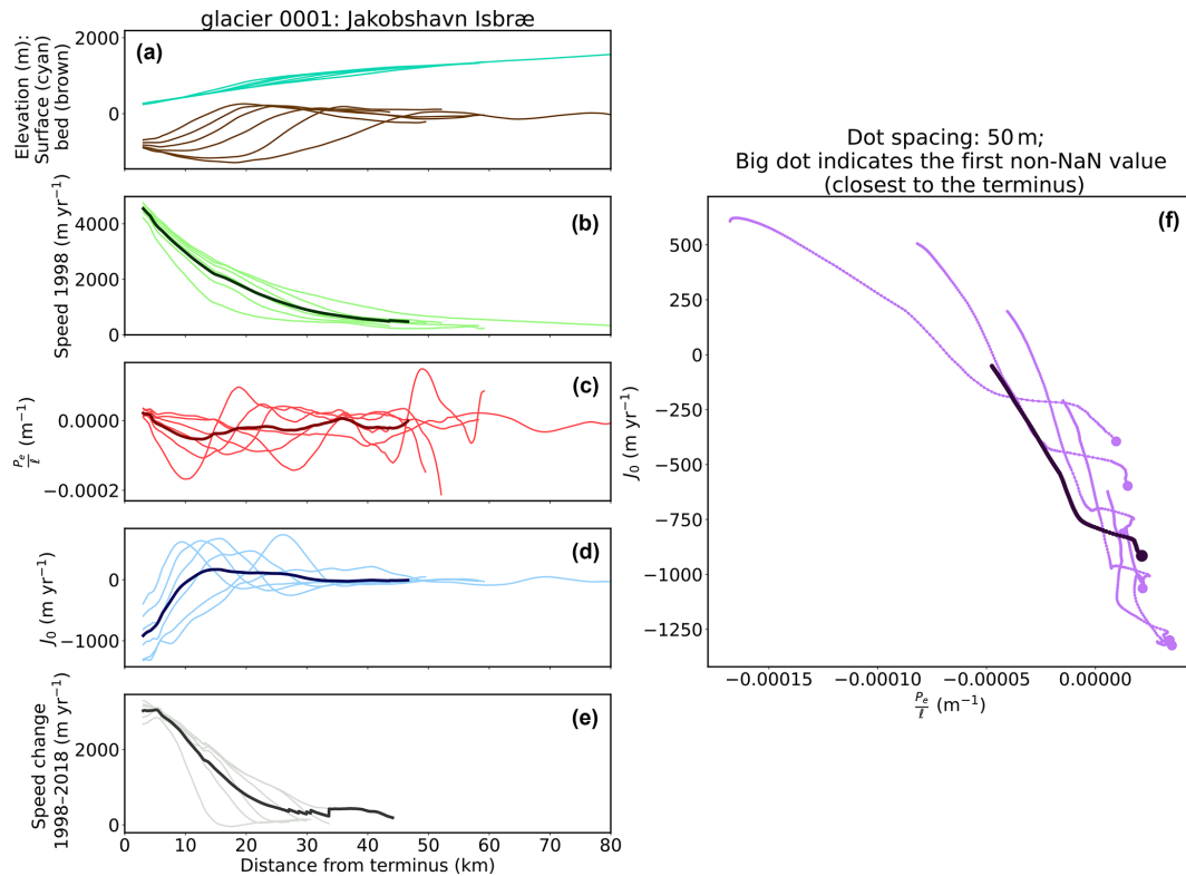
Figure 3. Example results from glacier 0001 (Jakobshavn Isbræ, 69.18° N, 49.76° W). (a) Surface elevation (cyan) and bed elevation (brown). (b) Surface speed in 1998. (c) Pe/l . (d) J_0 . (e) Speed change between 1998 and 2018. These plots show all six flowline profiles from a single basin in respect of the distance from the glacier terminus. The thick lines represent the average of these flowlines. (f) J_0 versus Pe/l along the first 10 km from the terminus. The big dots represent values at 3 km or the valid values closest to the terminus, and the small dots are plotted every 50 m along the flowline.
