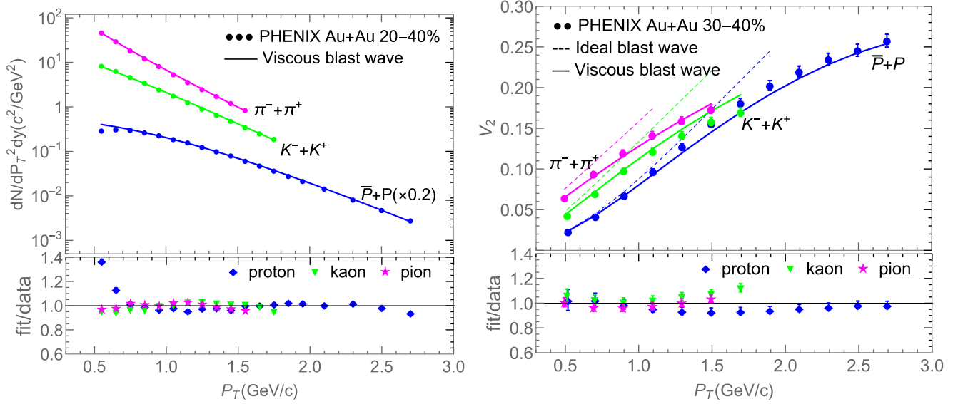
FIG. 5. Same as Fig. 2 for the PHENIX 30–40% centrality bin (20–40% for the spectrum). Statistical errors only are shown for PHENIX spectra.
