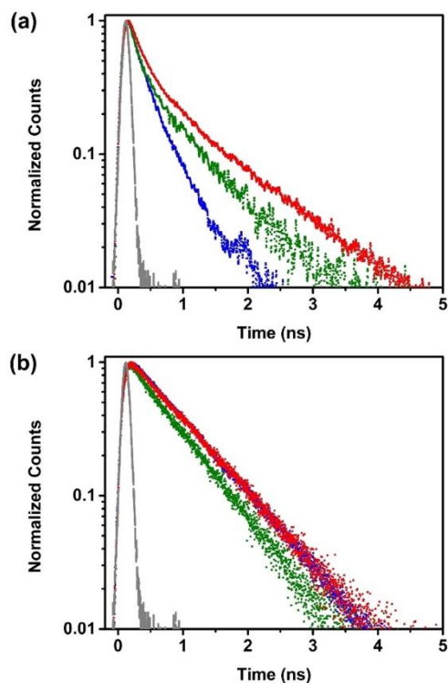
Figure 8. The fluorescence decay of IR140 detected at (a) S2 → S0 fluorescence maxima and (b) S1 → S0 fluorescence maxima in methanol (blue dots), ethylene glycol (green dots), and glycerol (red dots). The fluorescence lifetimes for (a) have been from the function f(t) = a_1 \exp(-t/\tau_1) + a_2 \exp(-t/\tau_2) while for (b) have been obtained from the function f(t) = -b_1 \exp(-t/\tau_3) + b_2 \exp(-t/\tau_4) . The time constants have been obtained post deconvolution of the IRF from the fluorescence decay signals. In both cases, the preexponential components are such that (a_1 + a_2 = 1 and b_1 + b_2 = 1) .
