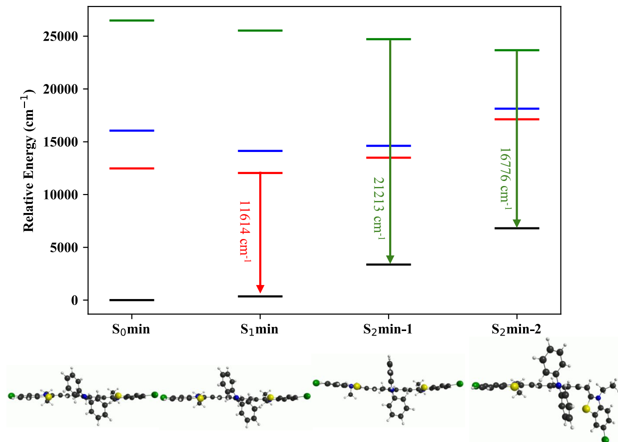
Figure 12. Computed state energies of IR140 in glycerol at corresponding geometries. S_0 , S_1 , S_1' , and S_2 energies are shown by black, red, blue and green lines, respectively. Energies for S_1 , S_1' , and S_2 are shifted as described in the text.
