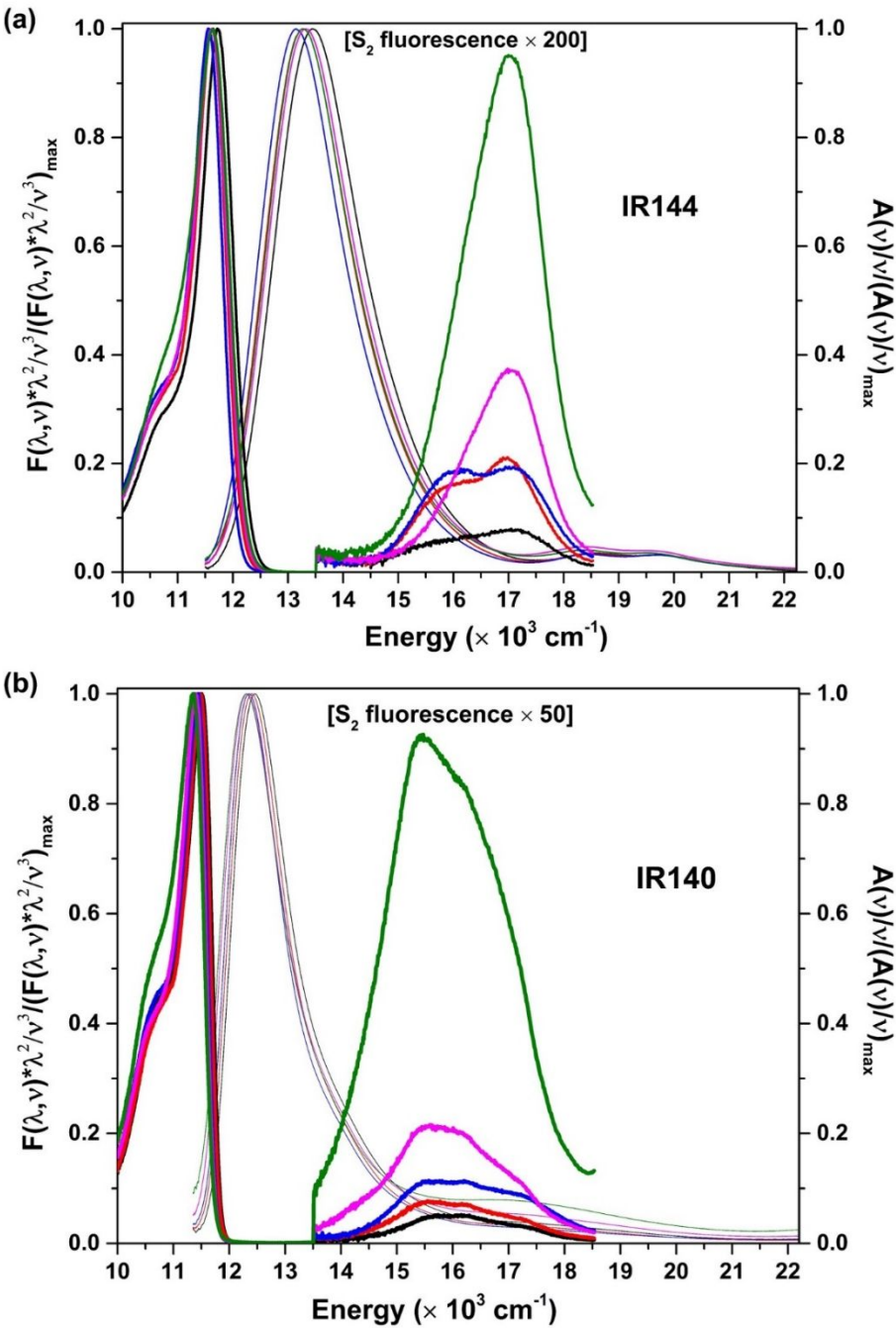
Figure 4. Steady-state absorption and fluorescence spectra for (a) IR144 and (b) IR140. The normalized absorption of both IR144 and IR140 is represented with thin lines whereas the normalized emission with thicker lines. Methanol, ethanol, n-propanol, ethylene glycol and glycerol are represented by black, red, blue, pink and green lines, respectively.
