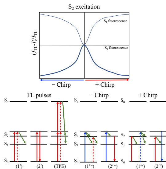
Figure 3. The interaction of chirped laser pulses with the S_2 state of a molecule. (top) Relative changes in fluorescence from the S_1 and S_2 states, (light and bold lines, respectively) as a function of chirp, according to ref. 5 (bottom) Albrecht ladder diagrams representing the laser-molecule interaction for TL and chirped pulses. Pathway (TPE) where two-photon excitation to an upper excited state S_n is accessible in this case, leading to enhanced S_2 fluorescence. Pathways ( 1^- and 1^+ ) are independent of chirp. Pathways ( 2^- ) is responsible for a decrease in fluorescence observed for negative chirp, however, non-radiative relaxation via IC leads to decreased S_2 fluorescence that is essentially symmetric with chirp sign. Solid/dashed arrows indicate ket/bra interactions. Blue/red arrows indicate high/low frequency portion of the spectrum. Green arrows indicate non-radiative transitions including wave-packet motion.
