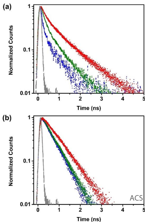
Figure 7. The fluorescence decay of IR144 detected at (a) S_2 \rightarrow S_0 fluorescence maxima and (b) S_1 \rightarrow S_0 fluorescence maxima in methanol (blue dots), ethylene glycol (green dots), and glycerol (red dots). The fluorescence lifetimes for (a) have been obtained from the function f(t) = a_1 \exp(-t/\tau_1) + a_2 \exp(-t/\tau_2) while for (b) have been obtained from the function f(t) = -b_1 \exp(-t/\tau_3) + b_2 \exp(-t/\tau_4) . The time constants have been obtained post deconvolution of the IRF from the fluorescence decay signals. In both cases, the preexponential components are such that (a_1 + a_2 = 1 \text{ and } b_1 + b_2 = 1) .
