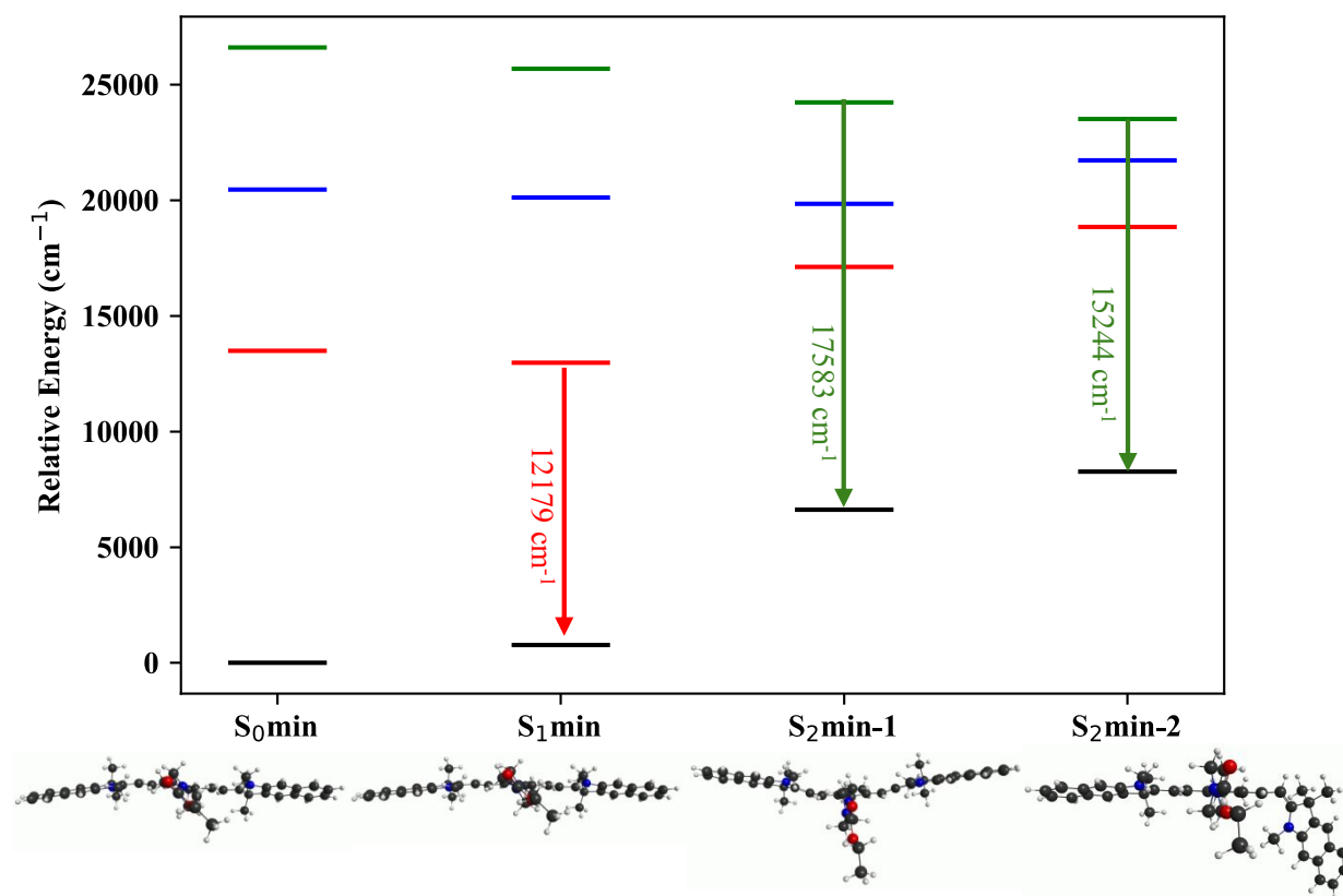
Figure 13. Computed state energies of IR144 in glycerol at corresponding geometries. S_0 , S_1 , S_1' , and S_2 energies are shown by black, red, blue and green lines, respectively. Energies for S_1 , S_1' , and S_2 are shifted as described in the text.
