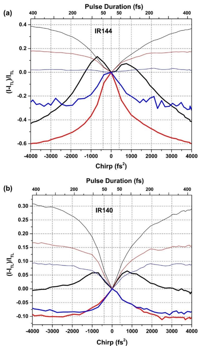
Figure 10. Chirp dependence scans carried out as a function of laser intensity for (a) IR144 and (b) IR140 in methanol. The thinner and thicker lines show the relative fluorescence intensity as a function of chirp compared to its TL value (I - I_{TL})/I_{TL} for S_1 and S_2 , respectively. Laser excitation power of 15mW, 10mW and 5mW are represented by black, red and blue lines, respectively. S_1 and S_2 data are represented by thin and thick lines, respectively.
