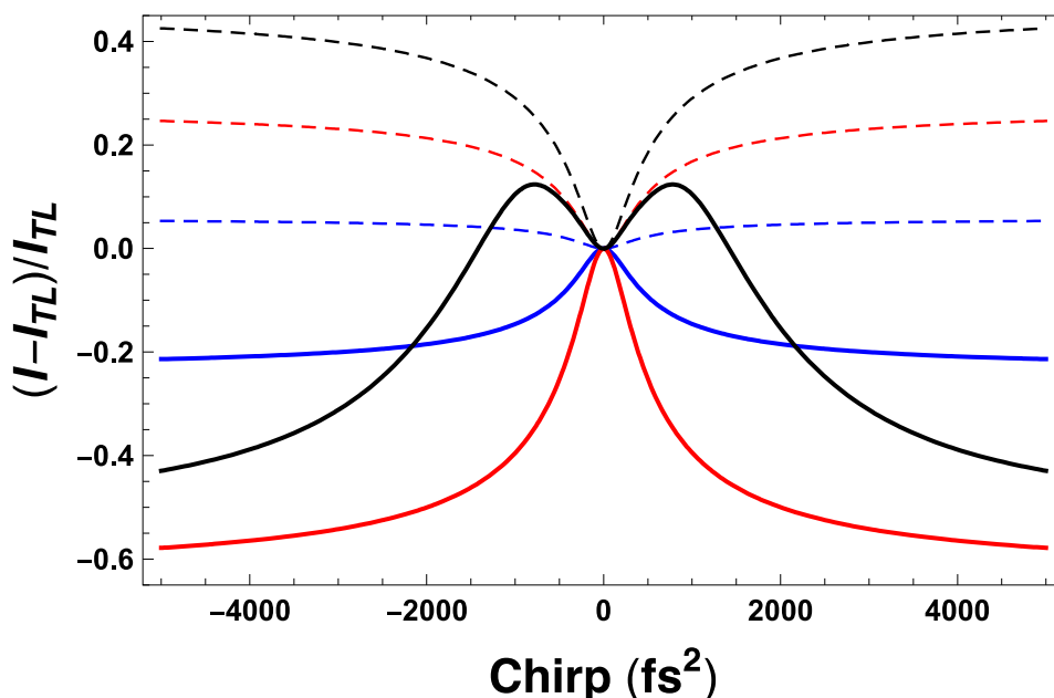
Figure 16. Results from numerical simulations of the S_1 and S_2 populations as a function of chirp for three different laser intensities: weak pulses (blue), higher intensity (red), and saturation (black); as described in the text.
