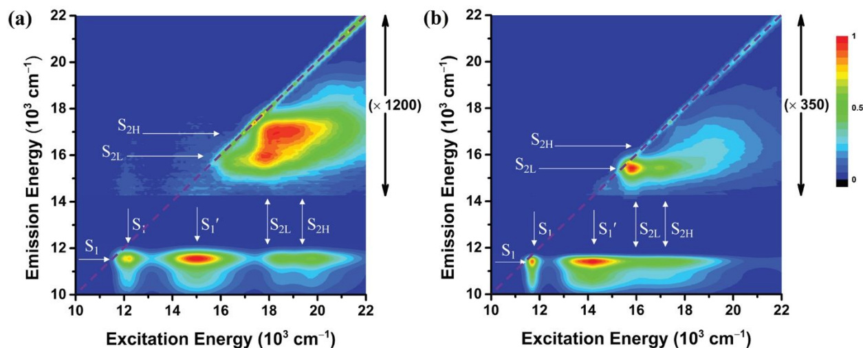
Figure 6. Excitation emission matrix spectra of (a) IR144 and (b) IR140 in n -propanol. The diagonal indicates scattered excitation light when both excitation energy and emission energy are equal.
