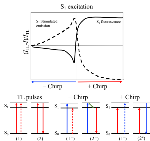
Figure 2. The interaction of chirped laser pulses with the S_1 state of a molecule. (top) Relative changes in fluorescence and stimulated emission from the S_1 state as a function of chirp (bold line and dashed line, respectively), according to ref. 24 (bottom) Albrecht ladder diagrams representing the laser-molecule interaction for TL and chirped pulses. Pathways (1^-) and (1^+) are independent of chirp, pathway (2^-) is responsible for the enhanced stimulated emission and decrease in fluorescence. Pathway (2^+) causes no effect because it is energetically forbidden. Solid/dashed arrows indicate ket/bra interactions. Blue/red arrows indicate high/low frequency portion of the spectrum. Green arrows indicate non-radiative transitions including wave-packet motion.
