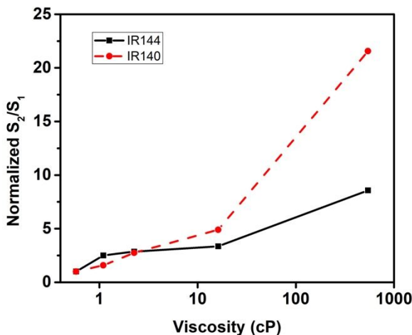
Figure 5. The integrated fluorescence ratio of S_2/S_1 from steady state spectra for IR144 and IR140 as a function of varying solvent viscosity (logarithmic scale). The numbers have been normalized such that the ratios are 1 for the respective methanol samples.
