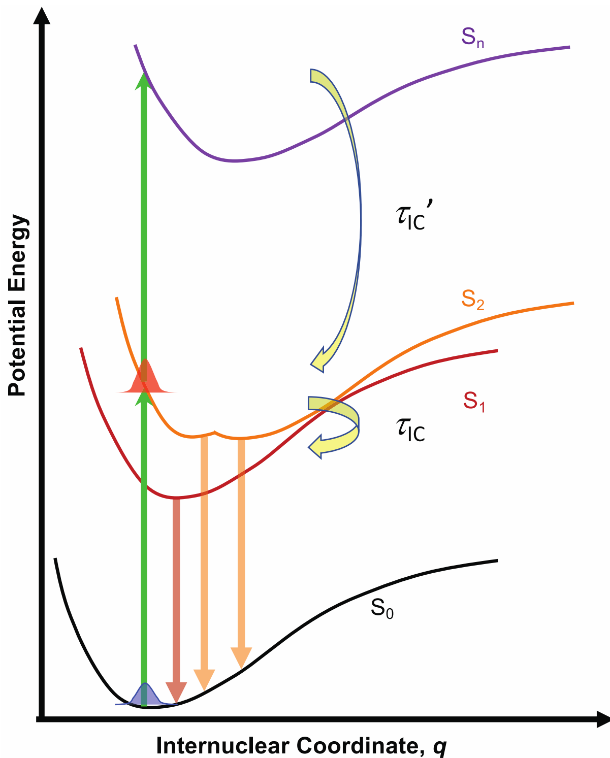
Figure 14. Schematic model representing potential energy curves that illustrate the different processes involved in the femtosecond chirped pulse experiments. As indicated in the theory section, two S_2 states were identified. The S_2 state
