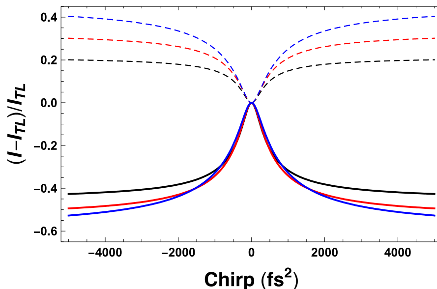
Figure 15. Results from numerical simulations of the S_1 and S_2 populations plotted as a function of chirp and viscosity. The viscosity of the solvent affects the rate k_2 , and this is reflected in the chirp dependence. Results shown for methanol (black), ethanol (red), and propanol (blue), where the only parameter changed in these simulations was the viscosity of the solvent.
