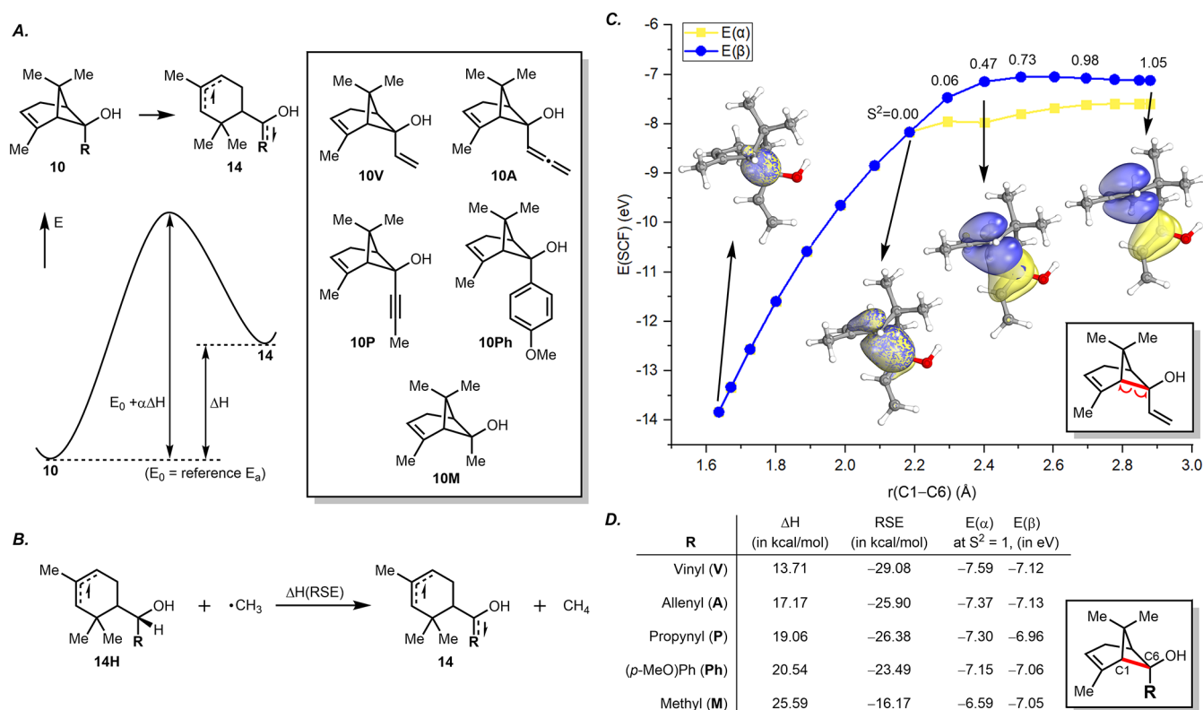
Figure 4. (A) Homolytic C–C bond cleavage of chrysanthanol derivatives to compare the relative barriers using the Bell–Evans–Polanyi principle. (B) The reaction scheme for the calculation of the radical stabilization energy (RSE). (C) Intrinsic bond orbital (IBO) profile of 10V along the intrinsic reaction coordinate for the formation of the diradical ( 10V → 14V ). E(\alpha) and E(\beta) represent the energies of the two radicals associated with the diradical intermediate. (D) Computed \Delta H , RSE, E(\alpha) , and E(\beta) values depending on the functional groups, R . Orbital energies were re-evaluated by the IBO exponent 2 orbital localization method based on the DFT calculation results using the B3LYP-D3/def2TZVP level of theory.
