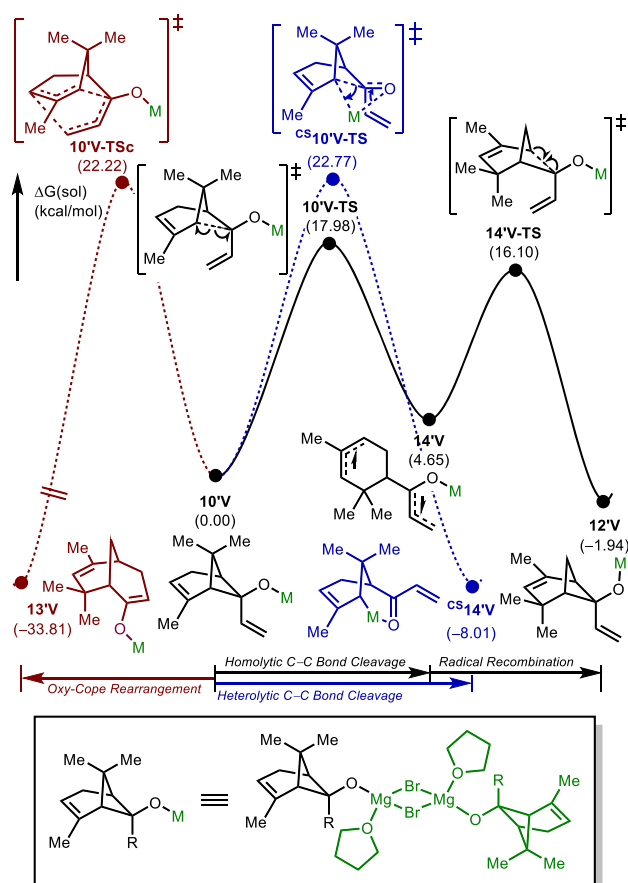
Figure 3. Free energy profile of plausible reaction pathways. The black trace represents the homolytic C–C bond cleavage and the blue dotted trace represents the heterolytic C–C bond cleavage. The red dotted line represents the oxy-Cope rearrangement. Geometry optimization and vibration energy calculations were conducted using DFT with the B3LYP-D3/6-31G** (LANL2DZ for Br) functional and basis set. Single-point energies were re-evaluated by the B3LYP-D3/6-311++G** (SDD for Br) level of theory in conjunction with a continuum solvation model using \epsilon = 7.4257 for THF.
