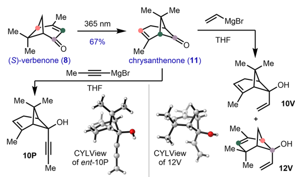
Scheme 1. Formation of Chrysanthenol Derivatives ( 10V and 10P ) and Rearranged [3.1.1]Bicycle ( 12V ) from ( S )-Verbenone ( 8 )
