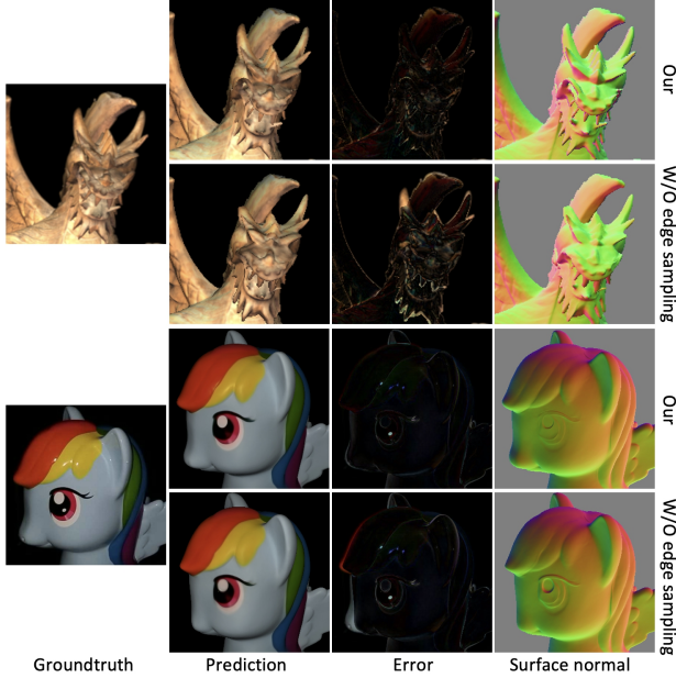
Figure 9. Ablations on our edge sampling algorithm using the synthetic dragon and real pony data. Without edge sampling, neural surface rendering performs poorly around edge regions, as shown by the error maps and surface normals.
