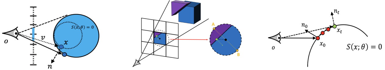
(a) Assuming known color, prior neural surface rendering methods [26, 39] fail to deform a small sphere to a target large sphere due to lack of edge handling.
