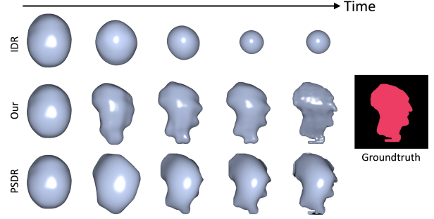
Figure 4. Given a single target image of an object with known color, we use an image loss to optimize a neural SDF with both IDR (top row) [39] and our IRON (middle row) method. We also optimize a mesh using PSDR (bottom row) [21]. Results show that IDR gets stuck due to not allowing SDF to deform along the image plane, while our method correctly optimizes the silhouette. PSDR can also handle the silhouettes, but the mesh quality degrades without intermediate remeshing steps.
