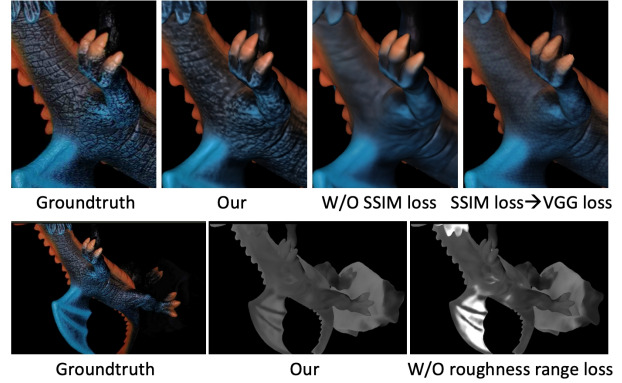
Figure 10. Ablations on our loss functions using the real dragon data. Without patch-based SSIM loss, our synthesized image is quite blurry, while VGG loss results in spurious texture details. The roughness range loss fixes issue of over-estimating roughness.
