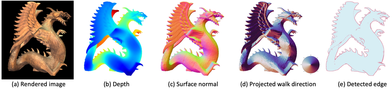
Figure 3. Demonstration of edge-aware surface rendering for neural SDF. To render the image (a), we first run sphere tracing to get the depth (b) and surface normal (c) corresponding to the pixel centers. We then localize subpixel-accurate edges by walking on the surface; the projected walk direction (d) is color-coded as shown in the inset color wheel. Detected edge pixels are shown in red in (e). We shade non-edge pixels as in existing neural surface rendering methods [26, 39], but shade edge pixels by accounting for the geometric discontinuity.
