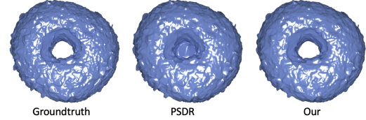
Figure 5. When using a mesh representation, it is difficult to design methods that can change the mesh topology in a differentiable way. In contrast, methods that use neural SDFs can more readily change their topology. Above, we use the mesh-based differentiable rendering pipeline PSDR [40] and our IRON pipeline to reconstruct this bagel by deforming an initial sphere. The results demonstrate that PSDR fails to recover the central hole, while our method has no such issue.
