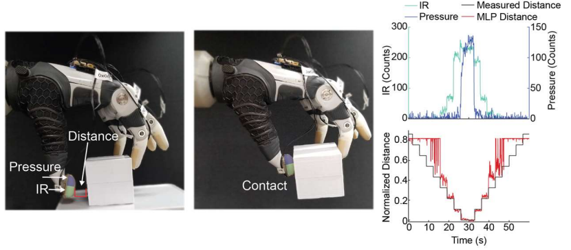
Figure 1: Labeled image of sensorized prosthetic hand (Left) and a subset of the training data used to create the autonomous controller (Right). Training data was collected using a cube, cylinder, and cone. The thumb was programmed to approach each object 20 times. Each approach consisted of incrementally moving the thumb forward, then waiting approximately 3 s before moving the thumb forward again. After contact, the thumb retracted from the object in a similar fashion. The autonomous controller is more accurate when the object is closer. That is, the predicted distance (red) more closely aligns with the ground-truth measured distance (black) as the distance becomes smaller.
