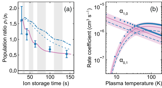
FIG. 4. (a) Population ratios p_1/p_0 corresponding to Fig. 3 (electrons applied in shaded time windows) with modeled evolutions starting from the measured populations at t = 28 s. Short-dashed, radiation only; dash-dotted, depletion by J -dependent DR also included; full line, additionally including inelastic collisions with the simplified \hat{\sigma}_{J,J'}(E) and fitting for \hat{\sigma}_{0,1}^0 . (b) Plasma rate coefficients \alpha_{1,0}(T) and \alpha_{0,1}(T) as constrained by the fitted \hat{\sigma}_{0,1}^0 (full lines and shaded one-sigma uncertainty), compared with R -matrix theory [11] (coalescing dots) and with the CB calculation (dashed line).
