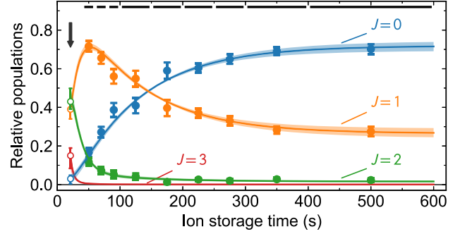
FIG. 2. Measured and modeled CH^+ rotational populations without electron interaction. Data p_J at t > 40 \text{ s} (filled symbols and one-sigma uncertainties) were determined from the signals S_J at the J -specific laser-probing wavelengths ( J \leq 2 ) averaged over the probing time windows indicated at the top (horizontal bars). Specialized laser scans (see the text) yielded populations \tilde{p}_J (unfilled symbols) at t = 21 \text{ s} (arrow) for J \leq 3 . With these as initial conditions, the radiative model was fitted to the later p_0 and p_2 ( p_1 follows as 1 - p_0 - p_2 ) varying T_{\text{low}} and \epsilon . Light colored bands: one-sigma uncertainties of the fitted model populations (including the \tilde{p}_J uncertainties).
