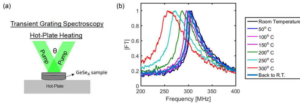
FIG. 13. TG measurement of elastic constant during temperature change on a hot plate. (a) Schematic of the experimental setup. (b) Rayleigh frequency shift with hot-plate temperature.
