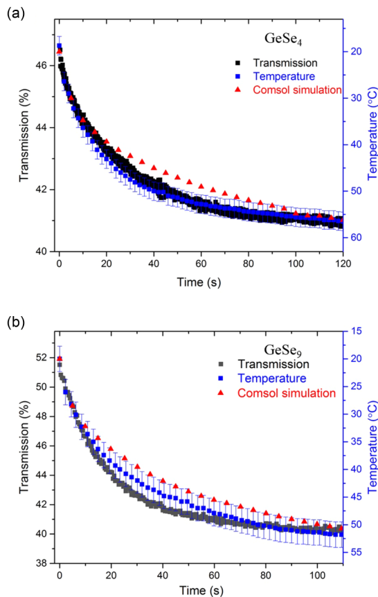
FIG. 9. Simultaneous change in transmission and temperature measured experimentally during laser irradiation with an intensity of 4.33 \text{ W/cm}^2 in (a) GeSe 4 glass, and (b) GeSe 9 glass, compared with the corresponding change in transmission predicted by COMSOL simulation.
