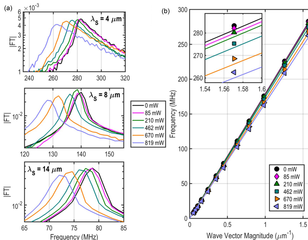
FIG. 6. TG measurement as a function of irradiation power in Ge-Se glass. (a) Shift in Rayleigh wave frequency with increasing irradiation power at different \lambda_s . (b) Dispersion curve showing the change in Rayleigh wave velocity (slope) as a function of irradiation power. The solid line denotes a linear best fit through the measured data points.
