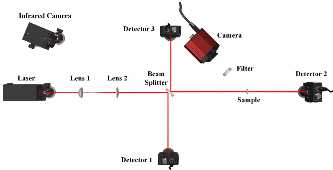
FIG. 1. Experimental setup for simultaneous measurements of transmission, reflection, photoexpansion, and surface temperature distribution of the Ge-Se glasses. A 2.5\times beam expander made of lens 1 and lens 2 generates an incident beam diameter of 2.1 mm. A spectral filter was applied in front of the camera to block the light of the laser wavelength.
