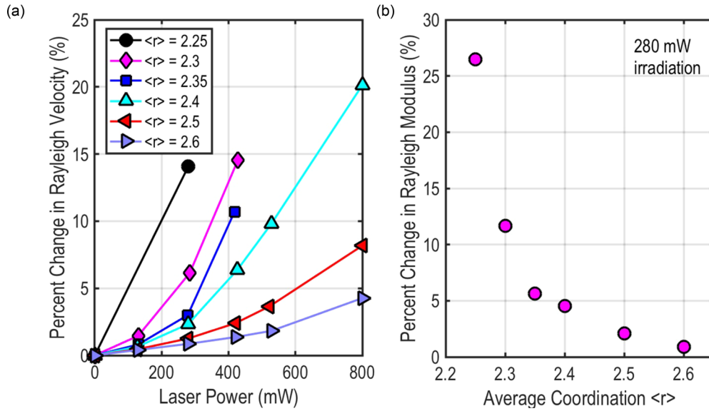
FIG. 7. Change in the Rayleigh elastic modulus with laser power for glasses across the Ge-Se system. (a) Percent change in Rayleigh wave velocity as a function of laser power for each glass composition. (b) Percent change in Rayleigh elastic modulus during irradiation with a power of 280 mW as a function of increasing bond density \langle r \rangle in the glass.
