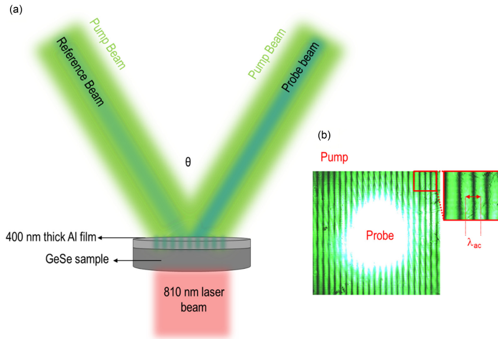
FIG. 2. (a) Schematic of the TG method used to measure change in elasticity during irradiation of Ge-Se glass. (b) Image of the interference fringe pattern created by the pump laser beams used to generate surface acoustic waves.
