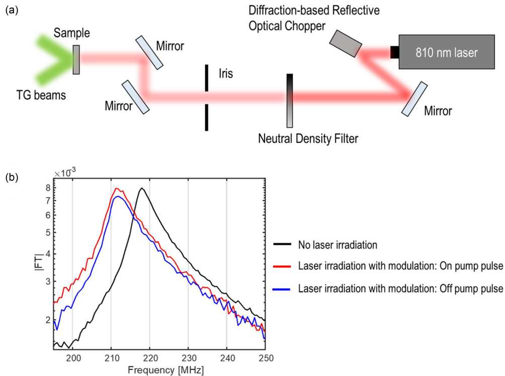
FIG. 8. TG measurement of elastic constant during rapid modulation of irradiation on and off using a diffraction-based optical chopper. (a) Optical setup. (b) Rayleigh wave frequency before irradiation (black line), during irradiation (red line), and 0.1 ms after turning off the irradiation (blue line).
