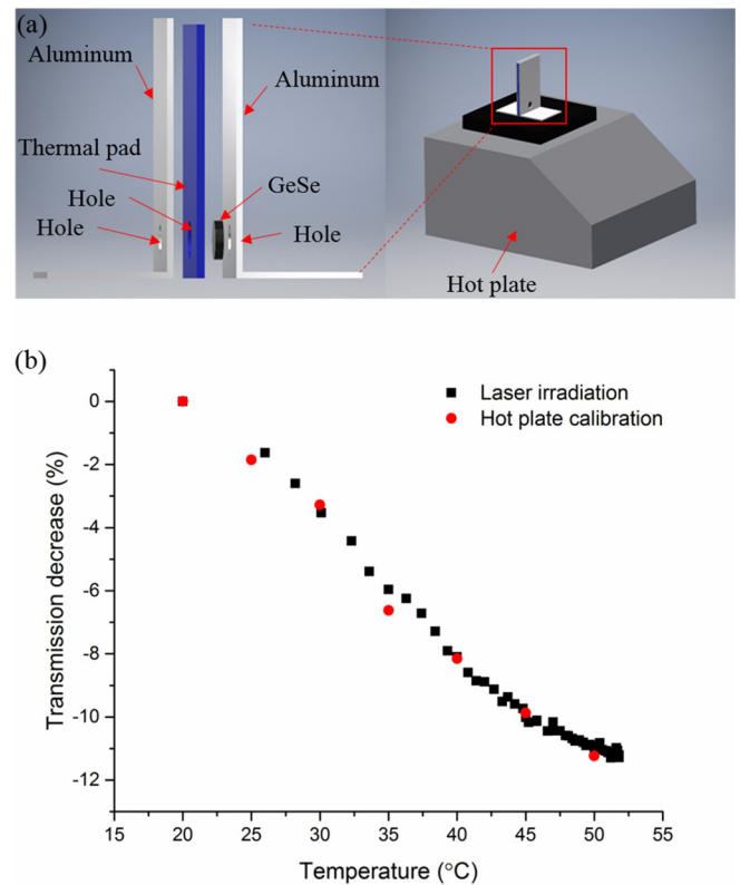
FIG. 10. (a) Experimental setup used to measure the change in transmission of Ge-Se glass disks as a function of temperature on a calibrated hot plate. (b) Decrease in transmission as a function of temperature for a GeSe 9 sample when the sample is heated on a hot plate compared to the change in transmission of the same sample with temperature measured by thermography under laser irradiation with an intensity of 4.33 \text{ W/cm}^2 .
