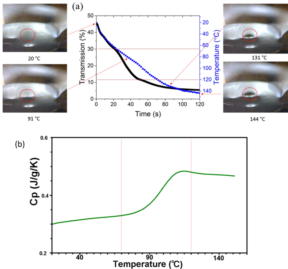
FIG. 12. (a) Correlation between photodarkening, temperature change, and photoexpansion monitored by optical microscopy during irradiation of a \text{GeSe}_9 glass with a power density of 9.15 \text{ W/cm}^2 . (b) Specific-heat capacity C_p of \text{GeSe}_9 measured by DSC as a function of temperature in the glass transition range. The onset of photoexpansion correlates with the onset of the glass transition measured by DSC where the glass becomes a supercooled liquid.
