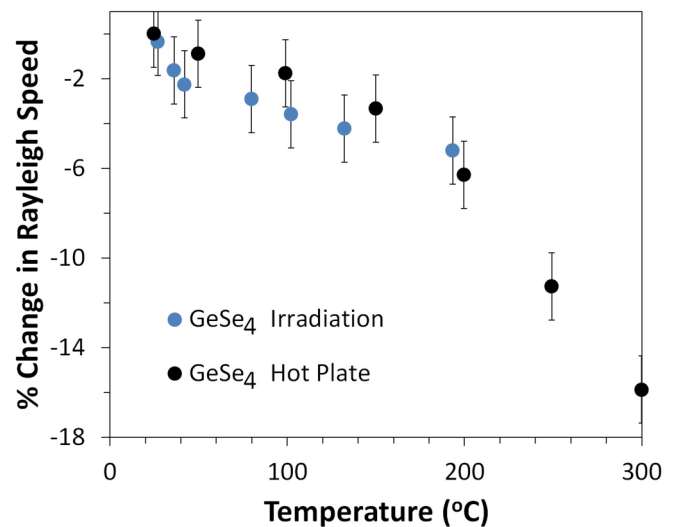
FIG. 14. Percent change in Rayleigh wave velocity of GeSe 4 during temperature change when the sample is heated on a hot plate compared to the change in Rayleigh wave velocity of the same sample during change in temperature measured by thermography under laser irradiation. The similarity in trend confirms that the laser-induced change in elasticity has a thermal origin.
