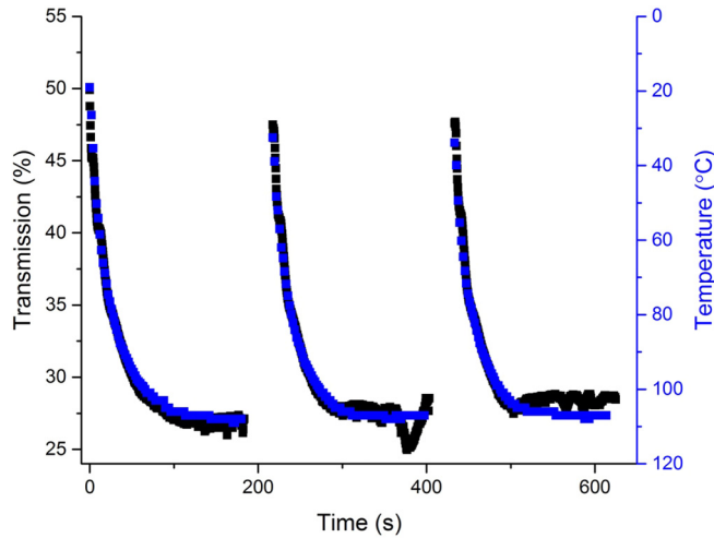
FIG. 11. Correlation between photodarkening recovery and temperature change over several cycles of light on and off in \text{GeSe}_4 .
