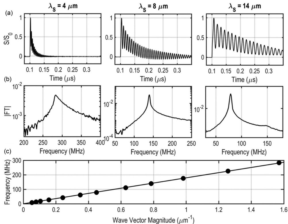
FIG. 3. (a) Surface wave oscillation measured in \text{GeSe}_4 at different SAW wavelength \lambda_s using the TG method. (b) The TG signal is Fourier transformed to identify the Rayleigh wave frequency. (c) A plot of frequency vs inverse wavelength yields the wave velocity in the material.
