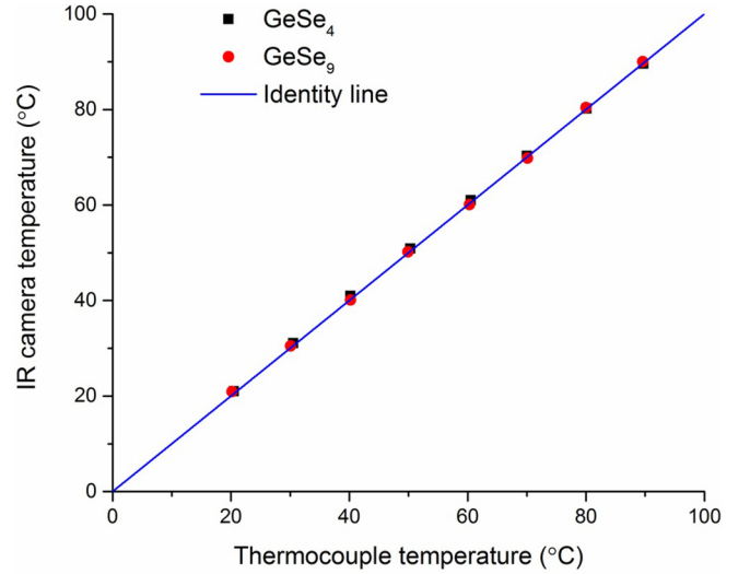
FIG. 5. Calibration curve showing the correlation between the temperatures measured by thermography and measured using a thermocouple for Ge-Se glasses coated with a polyimide film.
