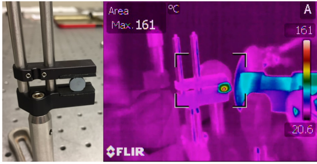
FIG. 4. (Left) Photo of a \text{GeSe}_4 chalcogenide glass disk mounted on a holder for simultaneous optical and thermal characterization. (Right) Infrared image corresponding to a frame of the movie recorded during irradiation. The temperature indicated corresponds to the maximum temperature of the irradiated spot located within the analysis frame.
