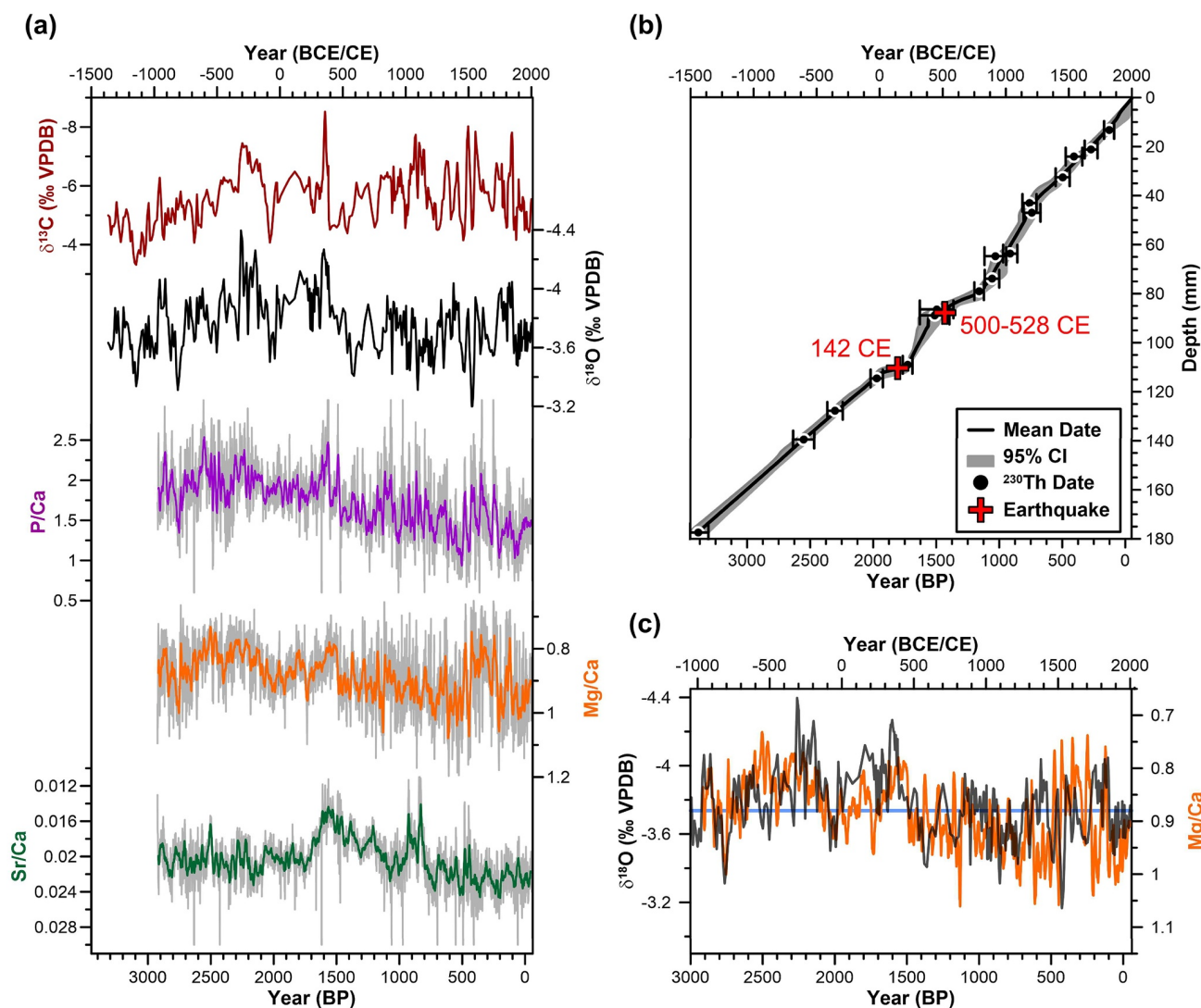
Figure 3. Stable-isotope (‰) and trace-element (mmol/mol -1 ) palaeoclimate proxy records from Kocain Cave. (a) Ko-1 proxies aligned so peaks represent wetter conditions. Trace-elements are displayed as annual (gray) and 15-year (colors) averages. (b) StalAge model for Ko-1. Earthquakes were not input to the model. (c) Comparison between Mg/Ca and \delta^{18}\text{O} ratios. Blue line represents the mean value of both records (0.88 mmol/mol -1 and -3.76‰).
