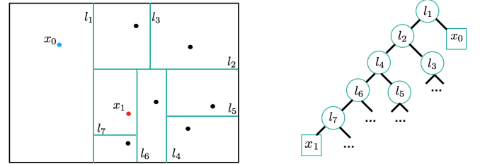
Figure 4: Finding outliers
