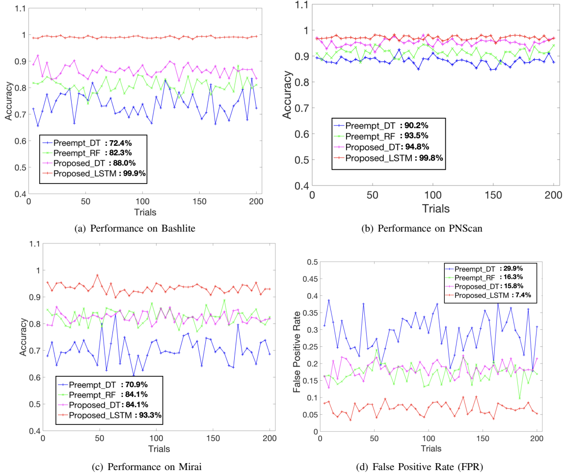
Figure 8: Performance of machine learning models: (a) - (c) for various malware, and (d) for benign benchmarks. The numbers in the legend box provides the average values for the four methods.
