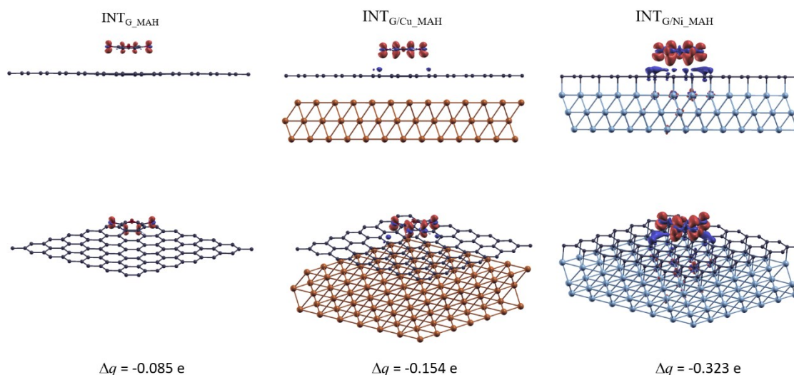
Figure 10. Charge density difference plots of \text{INT}_{\text{G}} , \text{INT}_{\text{G/Cu}} , and \text{INT}_{\text{G/Ni}} for MAH. Charge transfers ( \Delta q ) are determined from a Bader charge analysis of the electron densities.
