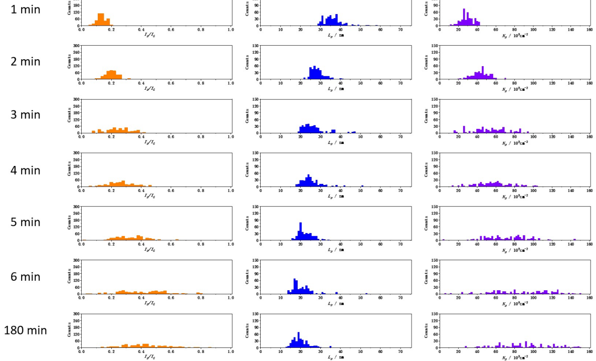
Figure 7. Histograms of Raman I_D/I_G (left), L_D (middle), and n_D (right) of (A) G/SiO 2 /Si, (B) G/Cu, (C) G/Ni after reacting with MAH at 150 °C for different lengths of time. For each set, ~400 data points were collected from 2 independent samples.
