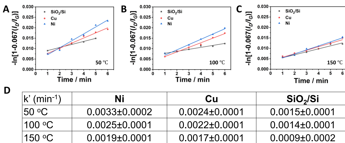
Figure 4. Plots of -\ln[1 - 0.067(I_D/I_G)] vs. time for reaction of DMBD with G/Ni (blue), G/Cu (red) or G/SiO 2 /Si (grey) at (A) 50 °C, (B) 100 °C, and (C) 150 °C. (D) The apparent rate constants ( k' , min -1 ) calculated from Eq. 3.
