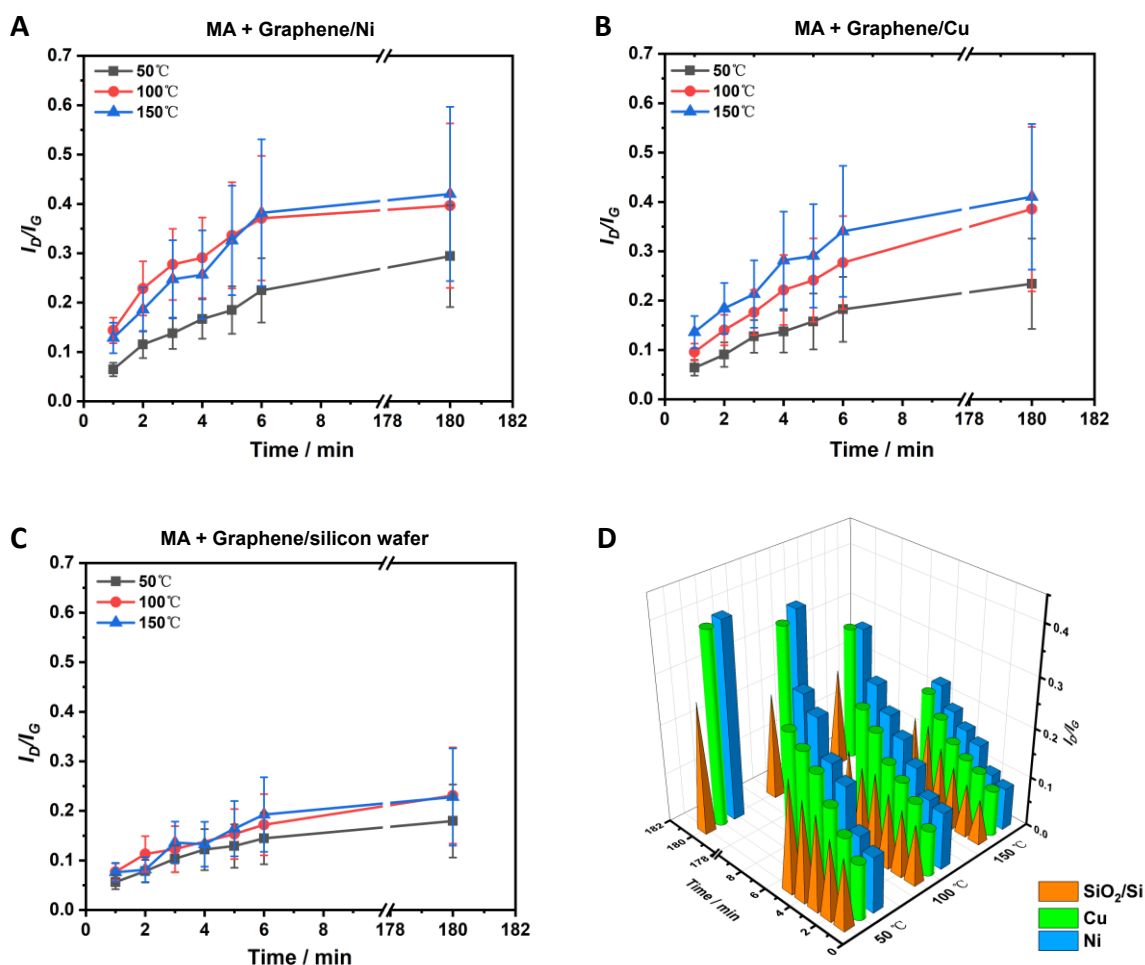
Figure 5. Raman I_D/I_G vs. reaction time at different temperatures for DA reactions between MAH and (A) G/Ni, (B) G/Cu, or (C) G/SiO 2 /Si. (D) 3D bar chart of I_D/I_G vs. reaction time and temperature. For G/Ni or G/Cu, the graphene films were transferred to silicon wafers prior to taking the Raman spectra. Data in (A) – (C) were collected from ~400 spots on 2 sets of independent samples.
