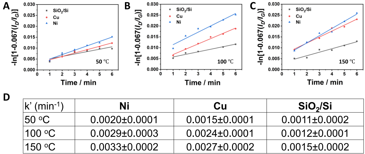
Figure 6. Plots of -\ln[1-0.067(I_D/I_G)] vs. time for reactions between MAH and graphene supported on Ni (blue), Cu (red) or silicon wafer (grey) at (A) 50 °C, (B) 100 °C, and (C) 150 °C. (D) The apparent rate constants ( k' , min -1 ) calculated from Eq. 3.
