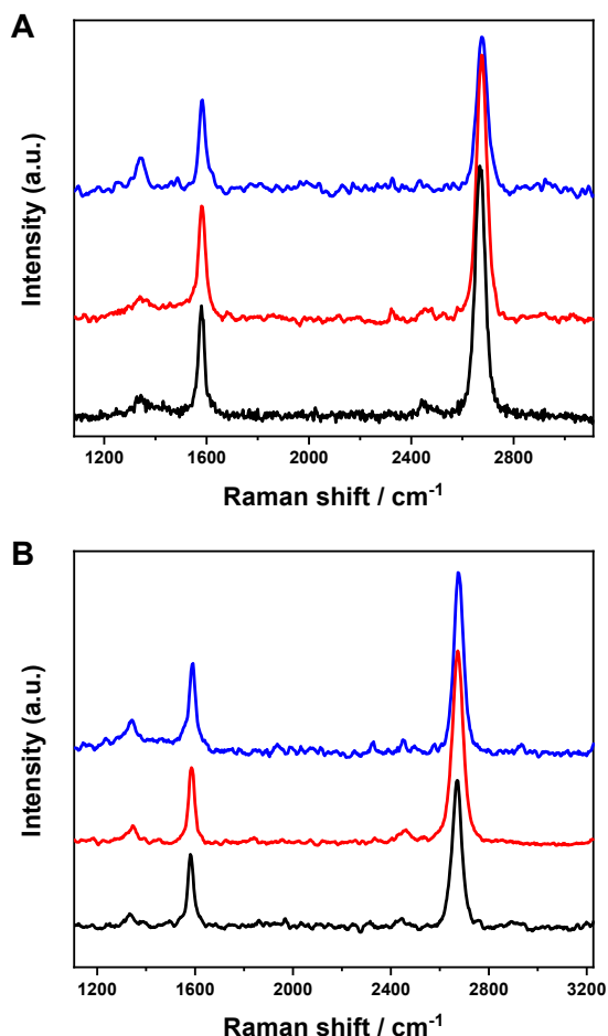
Figure 1. Representative Raman spectra of DA reactions on G/Ni (blue), G/Cu (red) or G/SiO 2 /Si (black): (A) DMBD at 50 °C for 5 min or (B) MAH at 100 °C for 5 min. For G/Ni or G/Cu, graphene was further transferred to silicon wafer for Raman characterization.
