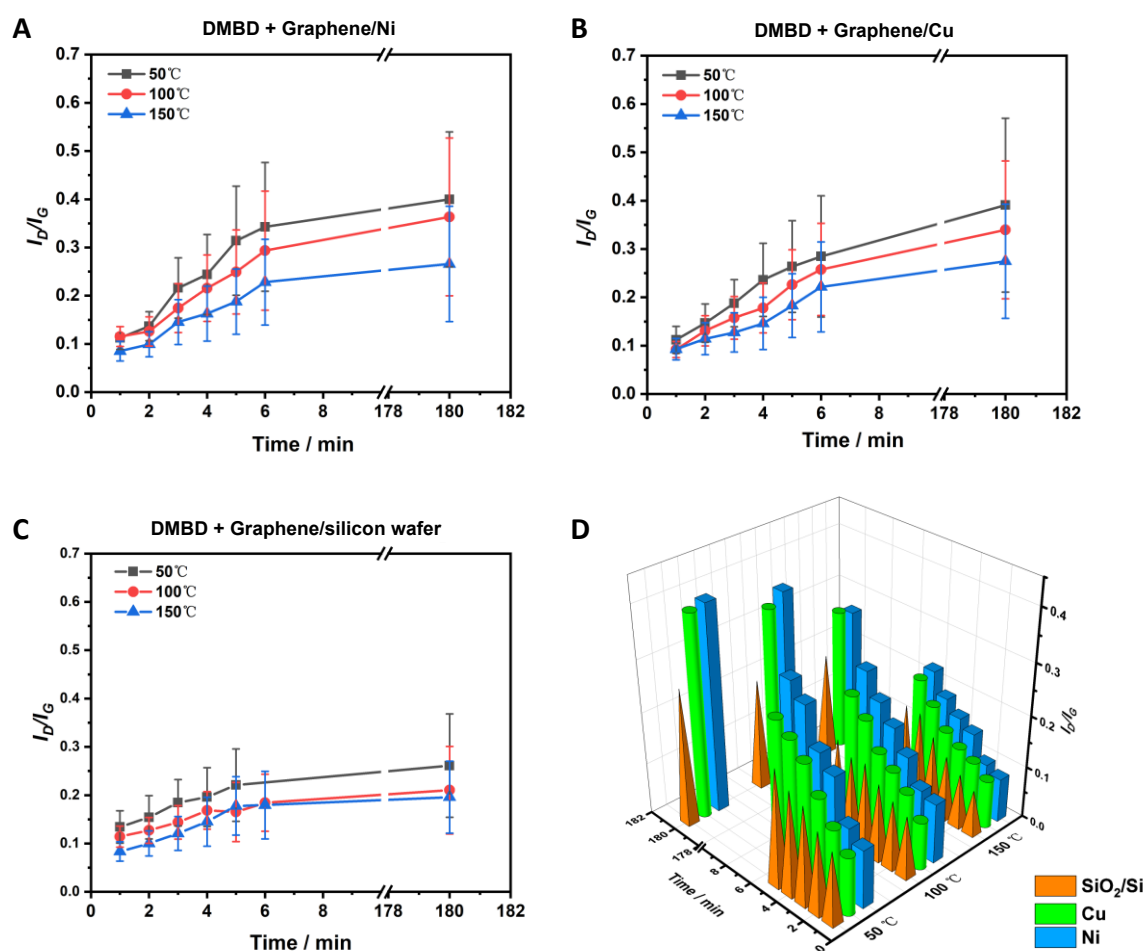
Figure 2. Raman I_D/I_G vs. reaction time at different temperatures for DA reaction between DMBD and (A) G/Ni, (B) G/Cu, or (C) G/SiO 2 /Si. (D) 3D bar chart of I_D/I_G vs. reaction time and temperature. For G/Ni or G/Cu, the graphene films were transferred to silicon wafers prior to taking the Raman spectra. Data in (A) – (C) were collected from ~400 spots on 2 sets of independent samples.
