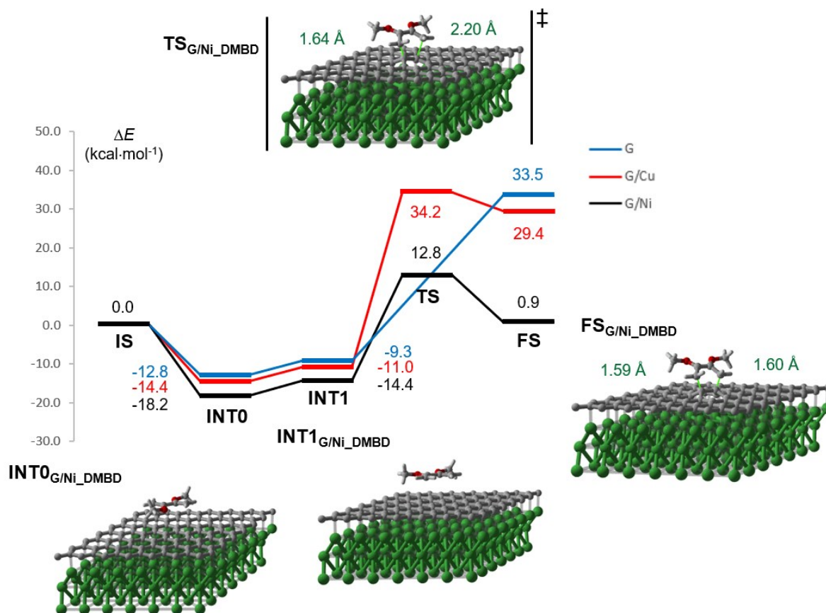
Figure 9. Reaction energy profiles for the Diels-Alder reaction using DMBD with G (blue), G/Cu (red) and G/Ni (black). Molecular representations for each G/Ni stationary point are given.
