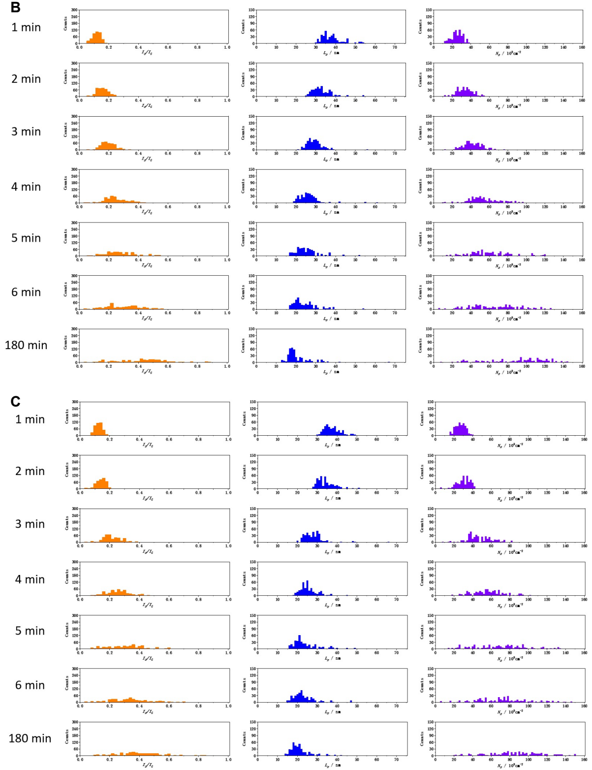
Figure 3. Histograms of Raman I_D/I_G (left) L_D (middle), and n_D (right) of (A) G/SiO 2 /Si, (B) G/Cu, (C) G/Ni after reacting with DMBD at 50 °C for different lengths of time. For each set, ~400 data points were collected from 2 independent samples.
