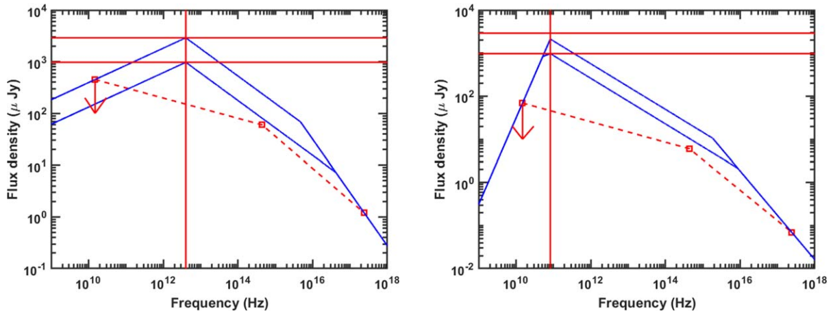
Figure 4. SED of the GRB 170202A fireball at the time of the first (left panel) and second (right panel) radio observations (see Figure 2). We indicate in red the constraints imposed by the model (see the text for the explanations) and in blue its limits.
