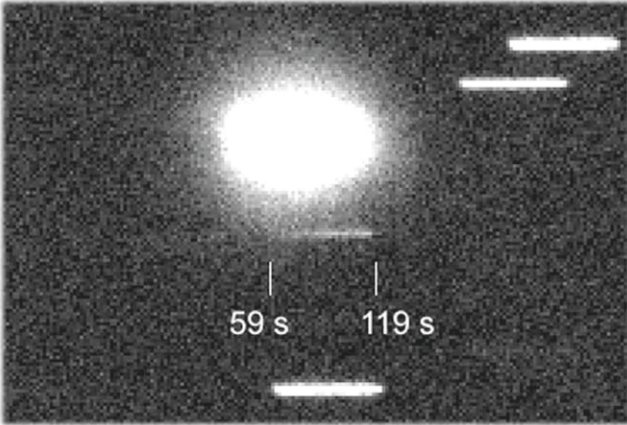
Figure 3. Trained image of GRB 170202A taken by Zadko. The rising part of its afterglow is clearly observed.
