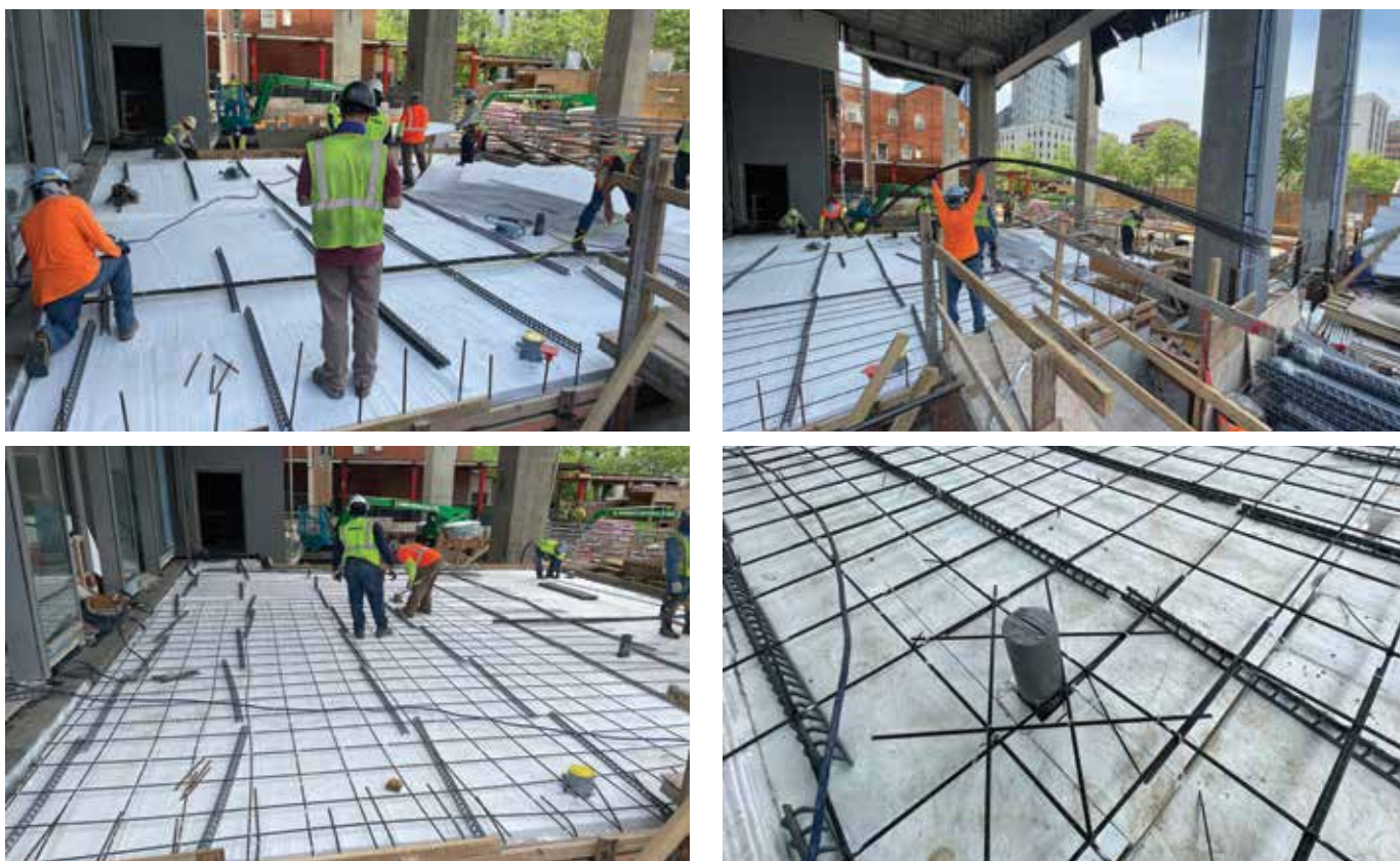
Fig. 4: Installation of No. 3 BFRP reinforcement for one of the topping slabs
