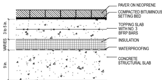
Fig. 2: Section of topping slab (Note: 1 in. = 25 mm)
