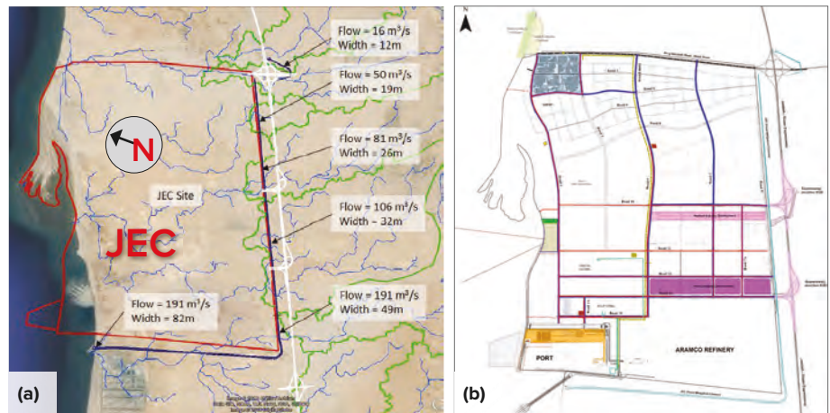
Fig. 2: JEC flood mitigation channel: (a) cumulative design flows and required widths; and (b) the channel passes the Aramco Refinery, located at the southeast corner of the site
