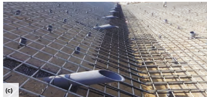
Fig. 7: The sloped sides of the JEC-FMC were tied to the base slab using bespoke splice bars: (a) a worker carries a bundle of splice bars; (b) prior to concrete placement, an overview of an upstream section of the JEC-FMC, showing grids, weep holes, and channel edge formwork; and (c) detail of lap splice at base-slope intersection
