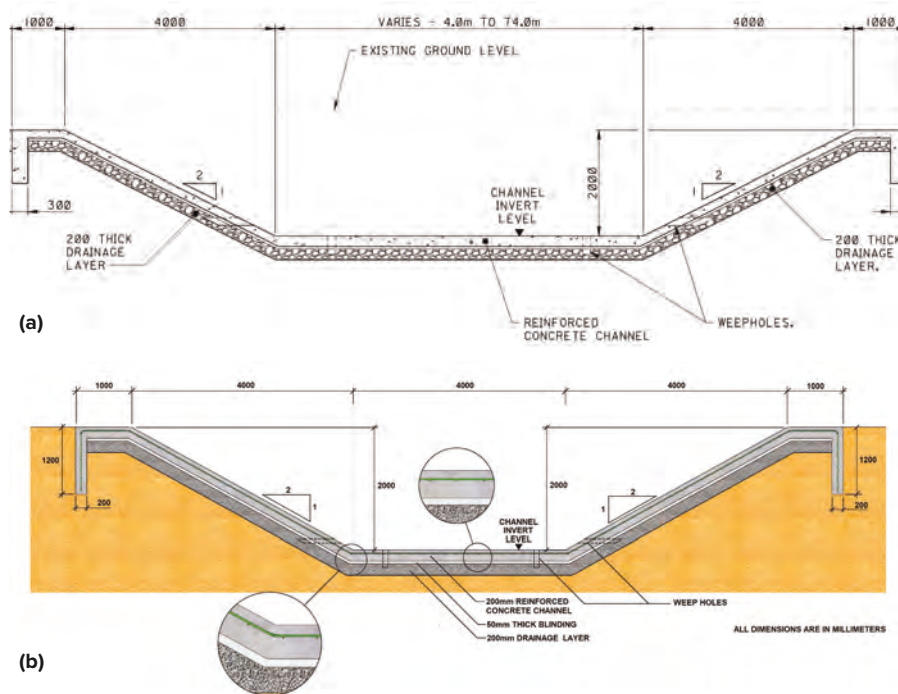
Fig 3: The flood mitigation channel: (a) cross section showing the original design with epoxy-coated steel (ECS) bars; and (b) cross section at the upstream end, showing the revised design with GFRP bars (Note: 1 m = 3.3 ft; 1 mm = 0.04 in.)
