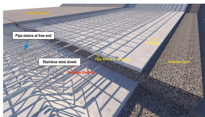
Fig. 4: Computer rendering of a typical transverse expansion joint
