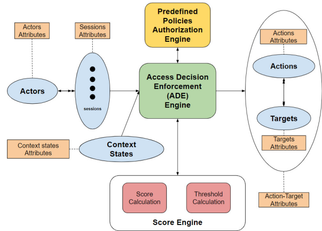
Figure 6: Zero Trust Score-based authorization framework (ZT-SAF)
