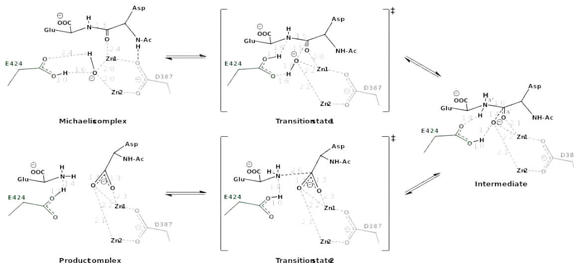
Scheme 1. wt-GCPII reaction mechanism, inferred from QM/MM modeling, X-ray crystallography, and site-directed mutagenesis. Note that the reaction mechanism was established in ref. 50 , whereas the distances are corrected based on our calculations.
