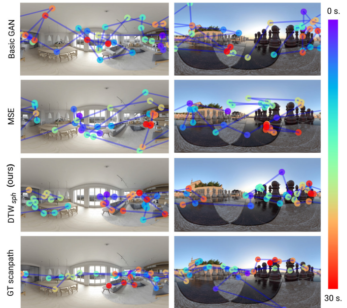
Fig. 7. Qualitative ablation results. From top to bottom : basic GAN strategy (baseline); adding MSE to the loss function of the former; our approach; and an example ground truth scanpath. These results illustrate the need for our DTW_{sph} loss term.
